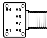
BOTTOM VIEW, HFBR 25x5A/B
