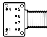
BOTTOM VIEW, HFBR-15x5x
