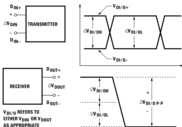
Figure 8. Differential signals.
