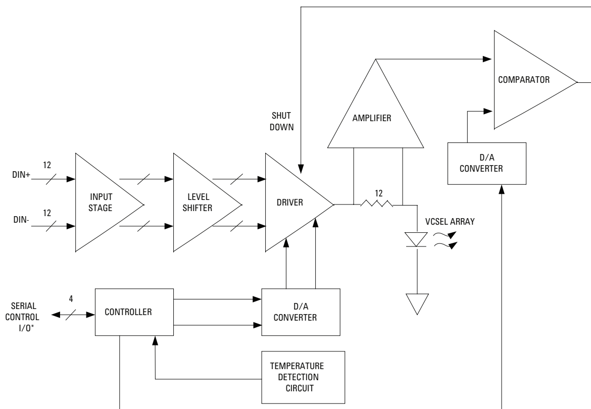
Figure 1. Transmitter block diagram.
