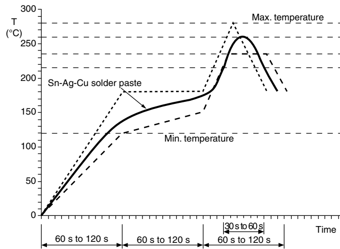
Fig. 8 - Soldering IR Reflow with SnAgCu Solder
