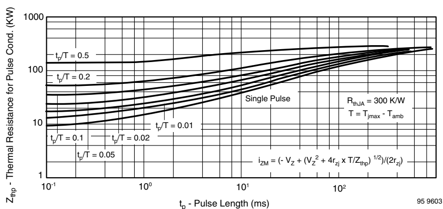
Fig. 10 - Thermal Response
