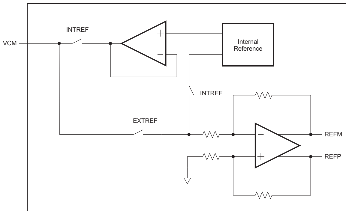
Figure 106. Reference Section
