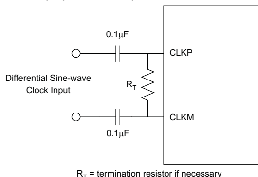
Figure 108. Differential Sine-Wave Clock Driving Circuit
