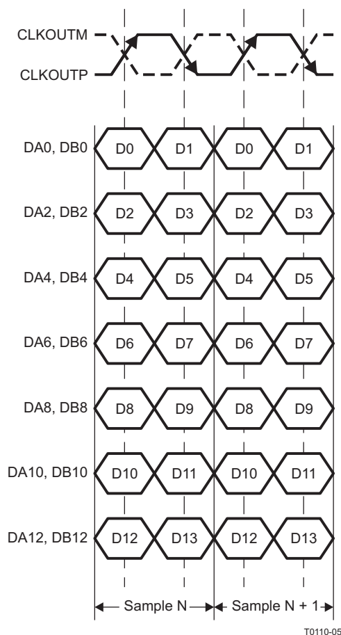
Figure 114. DDR LVDS Interface
