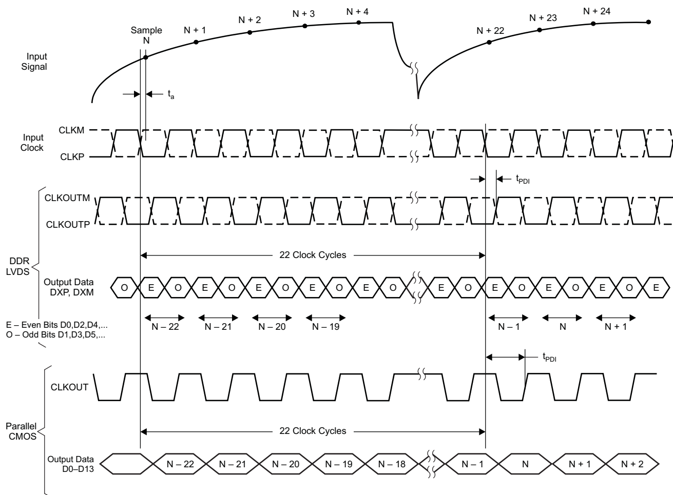
Figure 5. Latency Diagram
