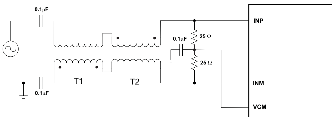
Figure 104. Drive Circuit with Very High Bandwidth (> 300 MHz)
