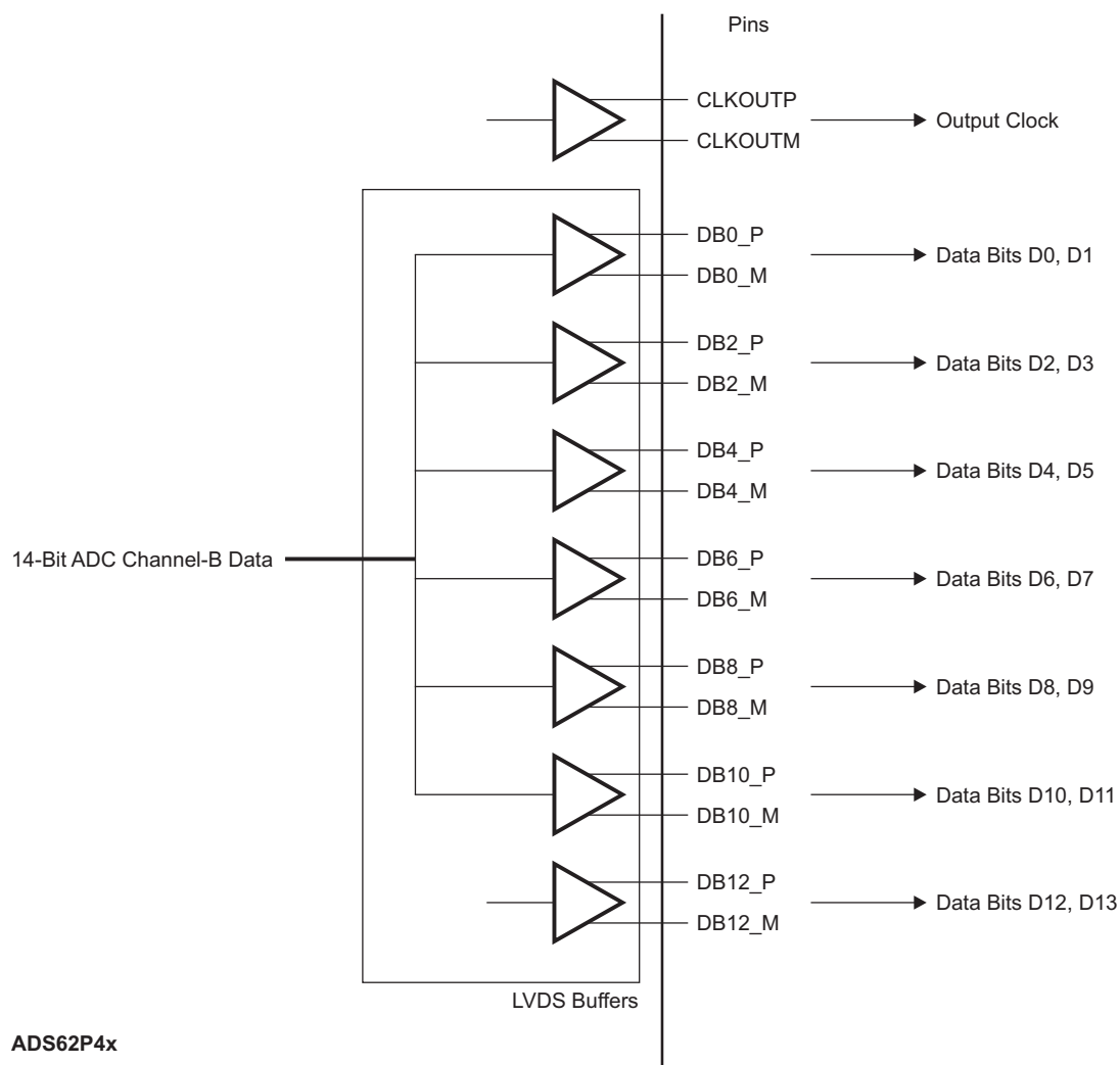
Figure 113. LVDS Outputs
