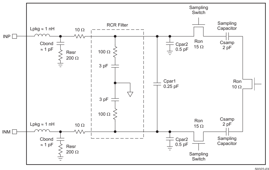
Figure 99. Analog Input Circuit
