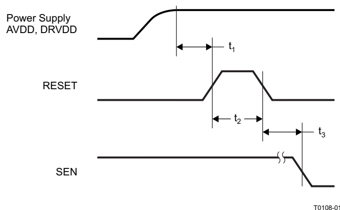
Figure 11. Reset Timing Diagram
