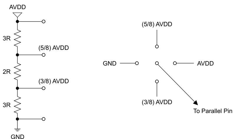
Figure 8. Simple Scheme to Configure Parallel Pins
