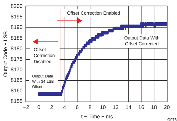
Figure 112. Time Response of Offset Correction
