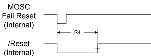
Figure 20-10. MOSC Failure Reset Timing
