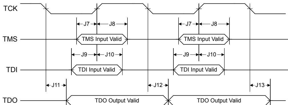
Figure 20-3. JTAG Test Access Port (TAP) Timing
