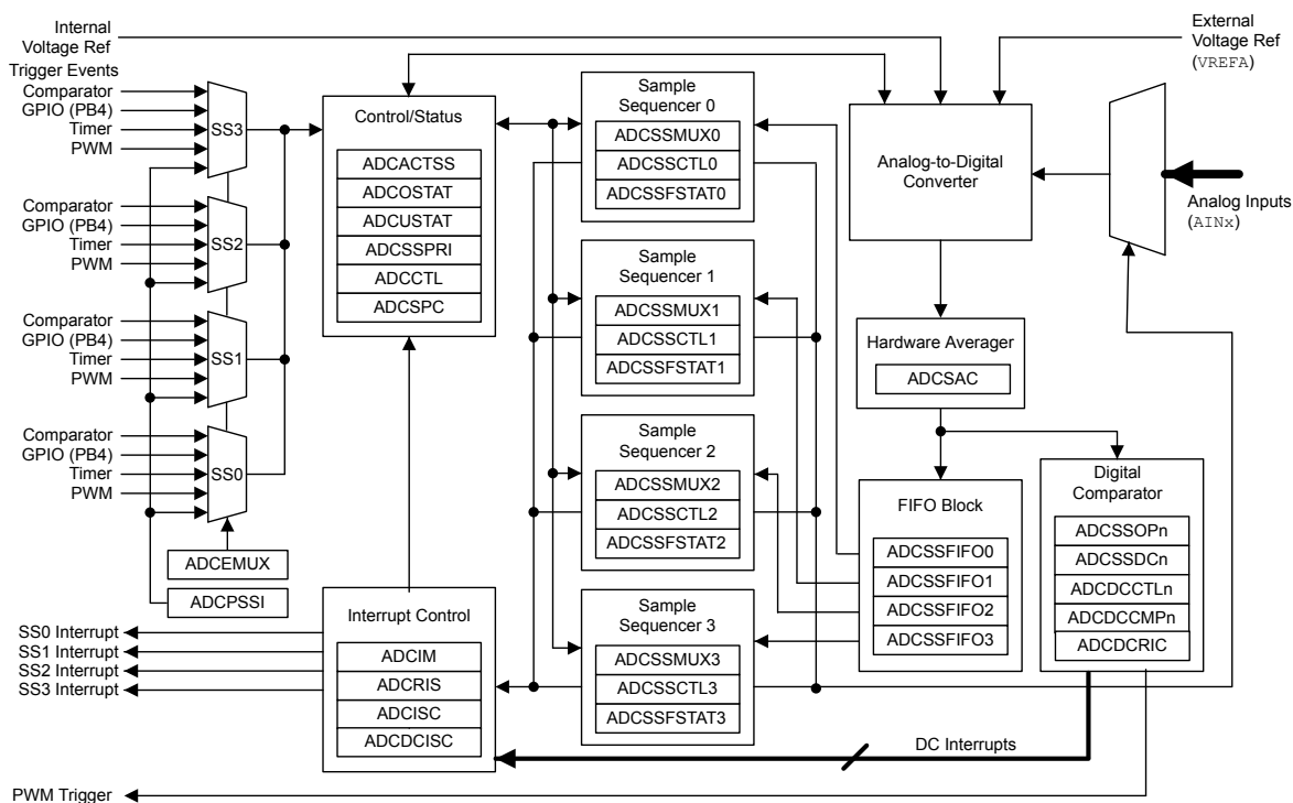
Figure 12-1. ADC Module Block Diagram
