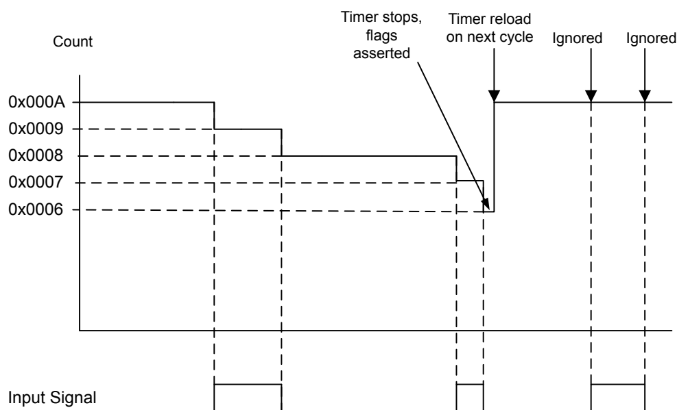
Figure 10-3. Input Edge-Count Mode Example
