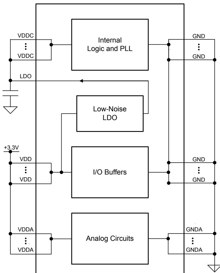
Figure 5-4. Power Architecture
