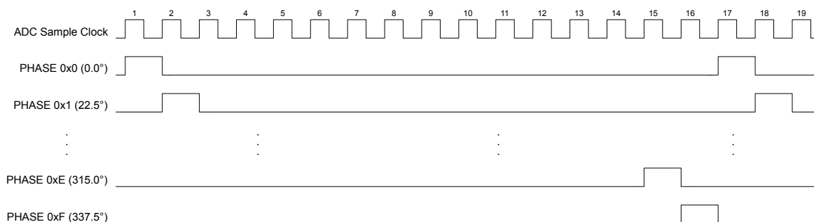
Figure 12-2. ADC Sample Phases
