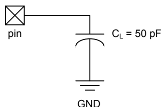
Figure 20-1. Load Conditions
