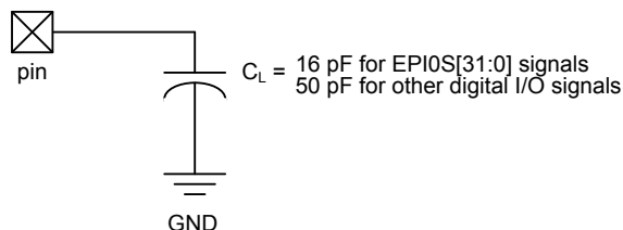
Figure 25-1. Load Conditions
