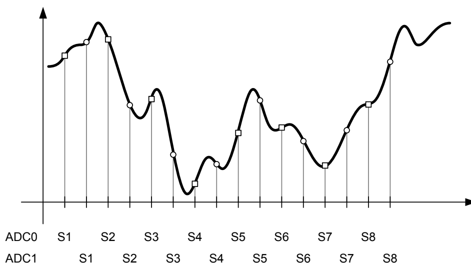
Figure 13-5. Skewed Sampling
