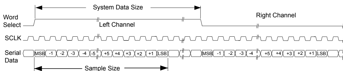
Figure 17-4. Right-Justified Data Transfer
