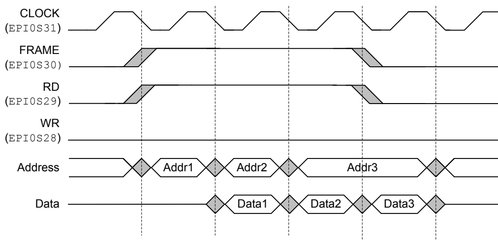
Figure 10-15. Read Accesses, FRM50=0, FRMCNT=0, RDCYC=1
