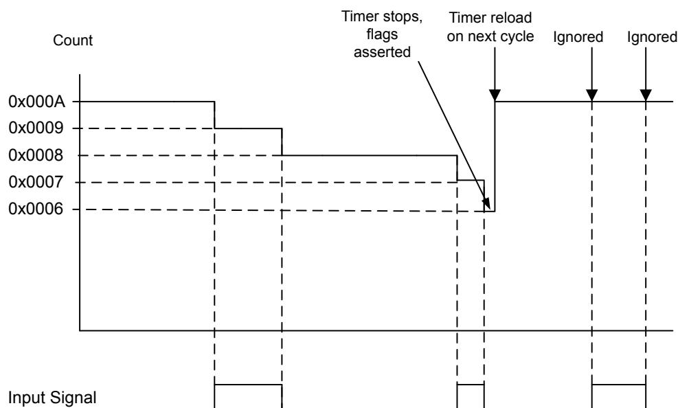
Figure 11-3. Input Edge-Count Mode Example
