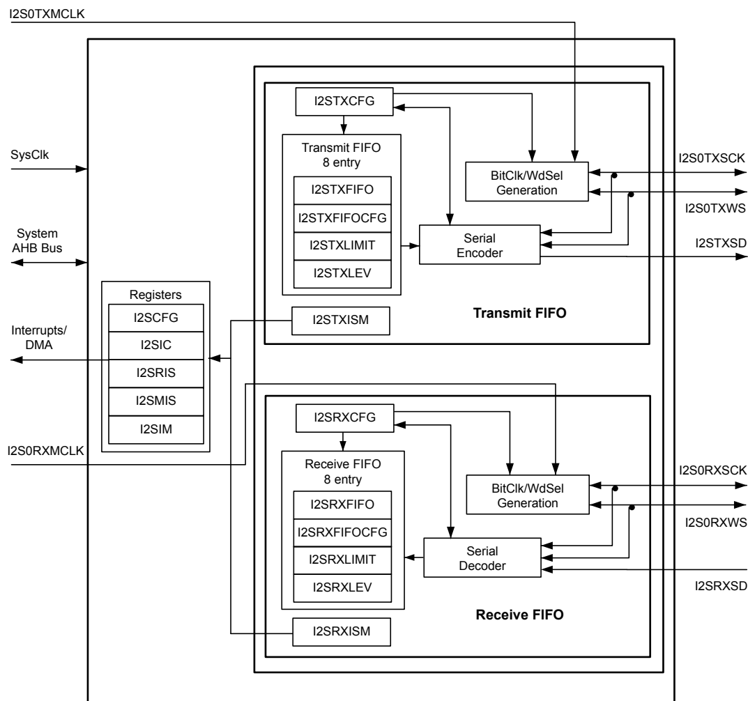
Figure 17-1. I 2 S Block Diagram
