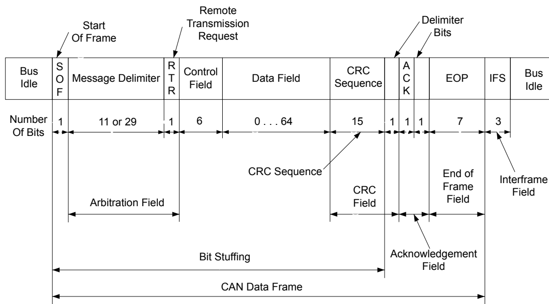
Figure 18-2. CAN Data/Remote Frame
