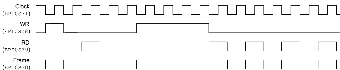
Figure 10-16. FRAME Signal Operation, FRM50=0 and FRMCNT=0
