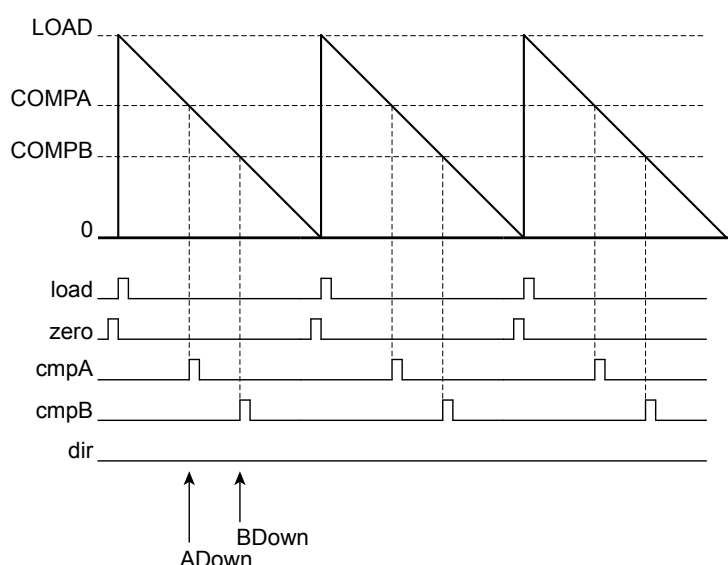
Figure 19-3. PWM Count-Down Mode
