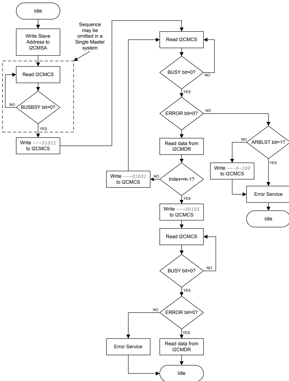
Figure 15-10. Master RECEIVE with Repeated START
