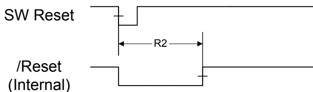
Figure 24-8. Software Reset Timing
