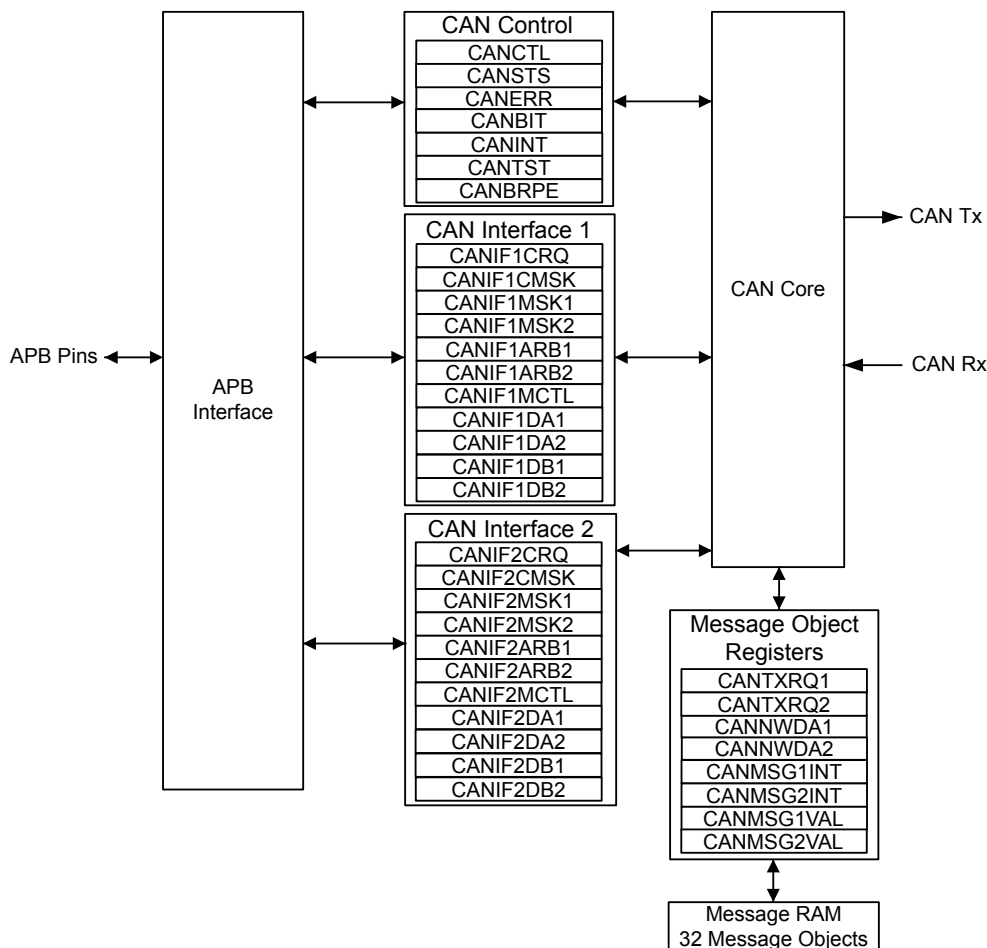
Figure 16-1. CAN Controller Block Diagram
