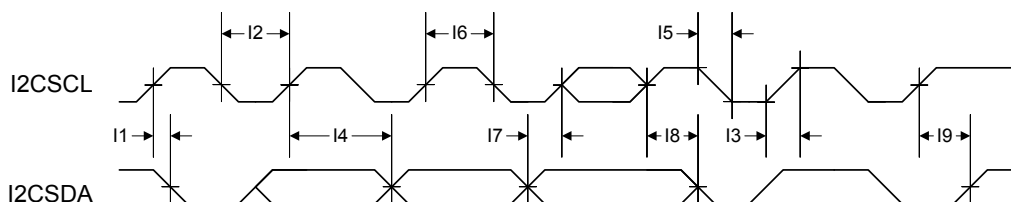
Figure 24-17. I 2 C Timing
