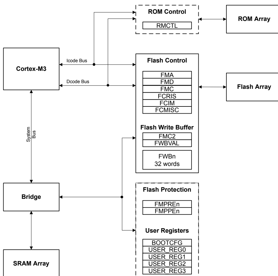
Figure 7-1. Internal Memory Block Diagram
