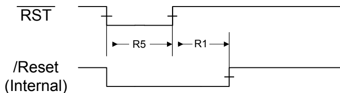
Figure 24-7. External Reset Timing ( \overline{\text{RST}} )
