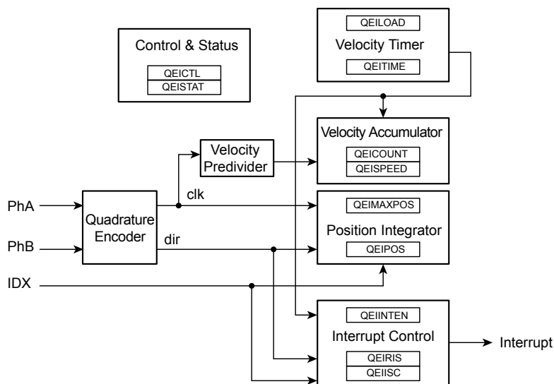
Figure 20-1. QEI Block Diagram
