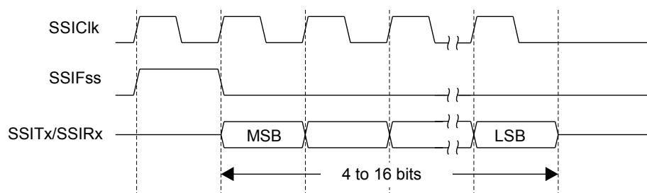
Figure 14-2. TI Synchronous Serial Frame Format (Single Transfer)
