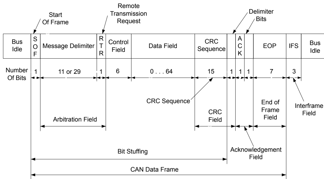
Figure 16-2. CAN Data/Remote Frame
