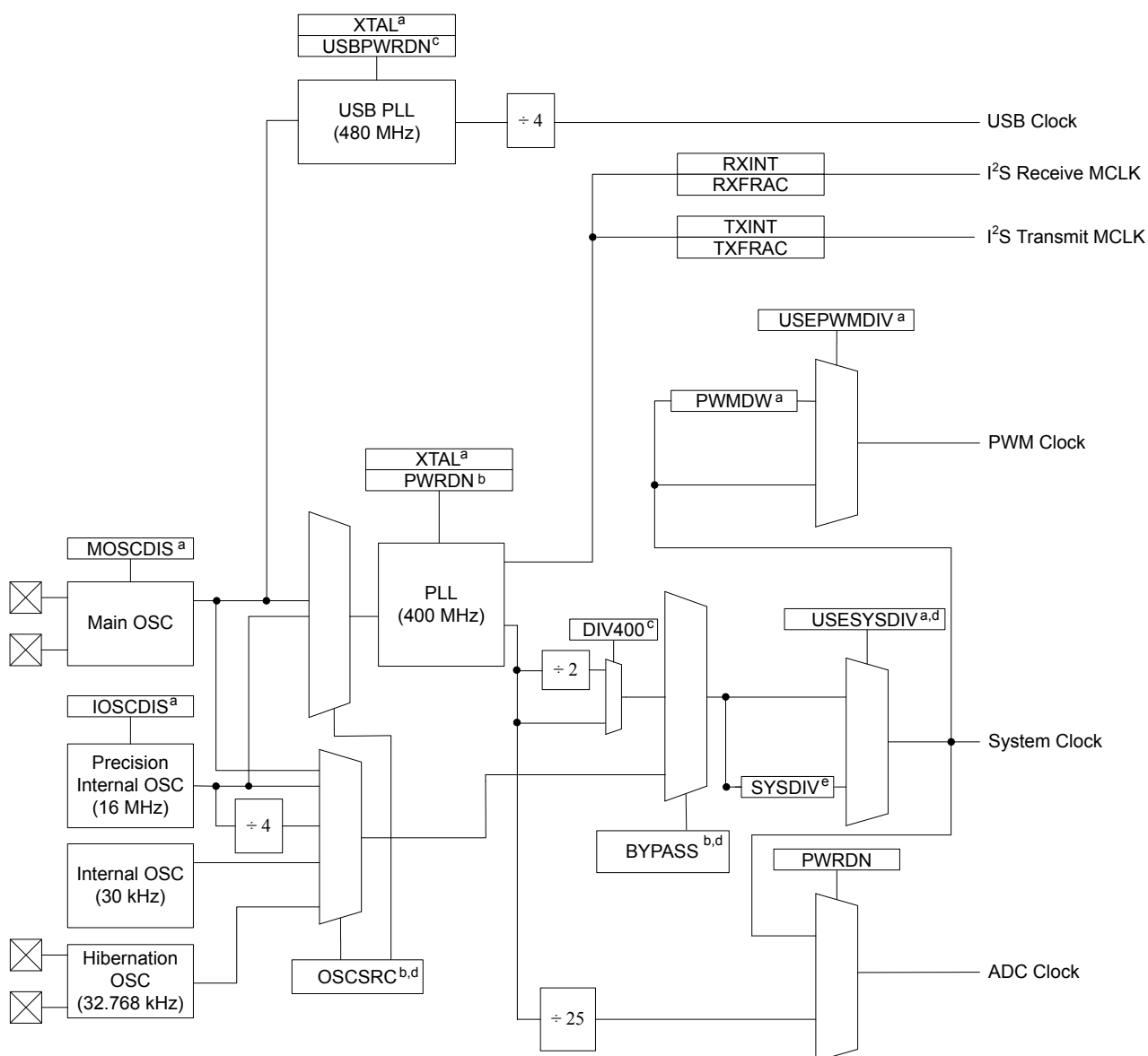
Figure 5-5. Main Clock Tree
