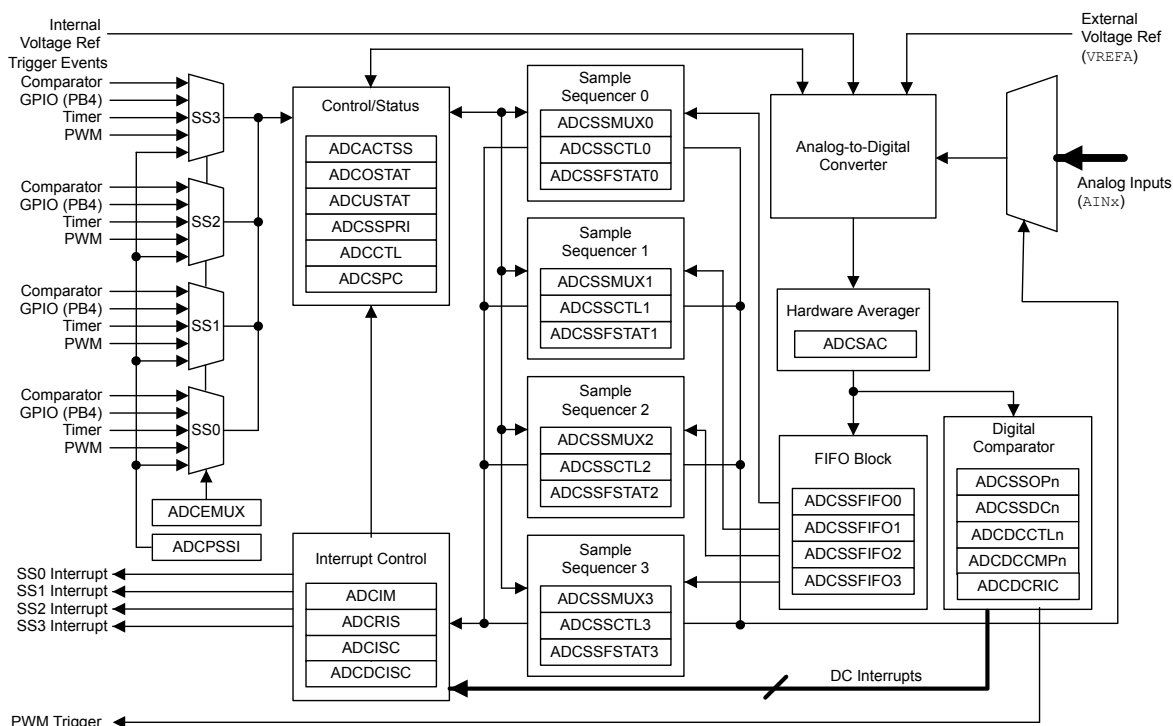
Figure 12-2. ADC Module Block Diagram
