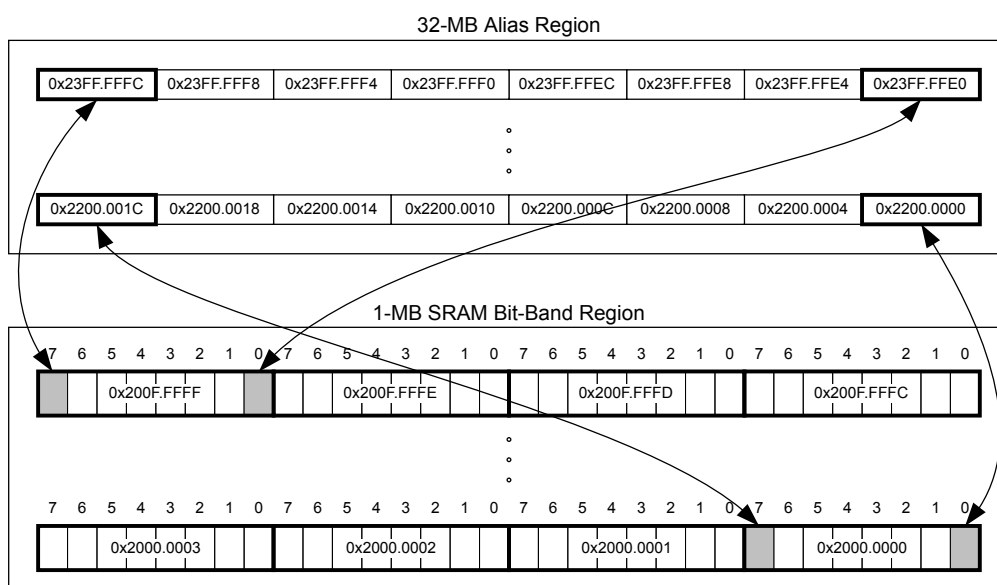
Figure 2-4. Bit-Band Mapping
