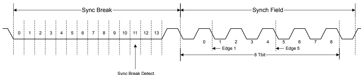
Figure 13-5. LIN Synchronization Field
