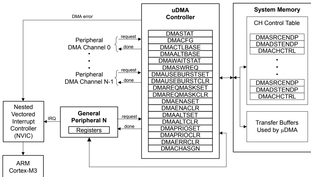
Figure 8-1. \mu DMA Block Diagram
