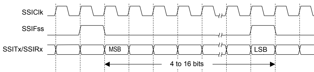
Figure 14-3. TI Synchronous Serial Frame Format (Continuous Transfer)
