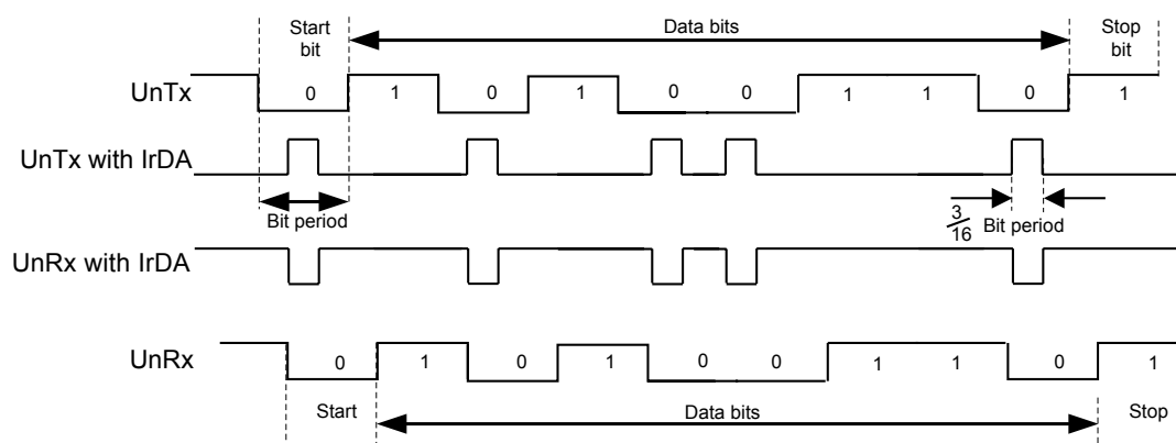
Figure 13-3. IrDA Data Modulation
