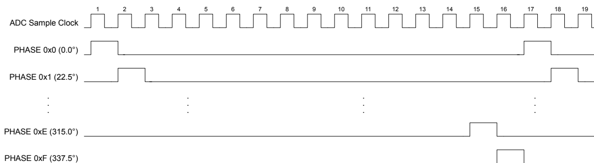
Figure 12-3. ADC Sample Phases
