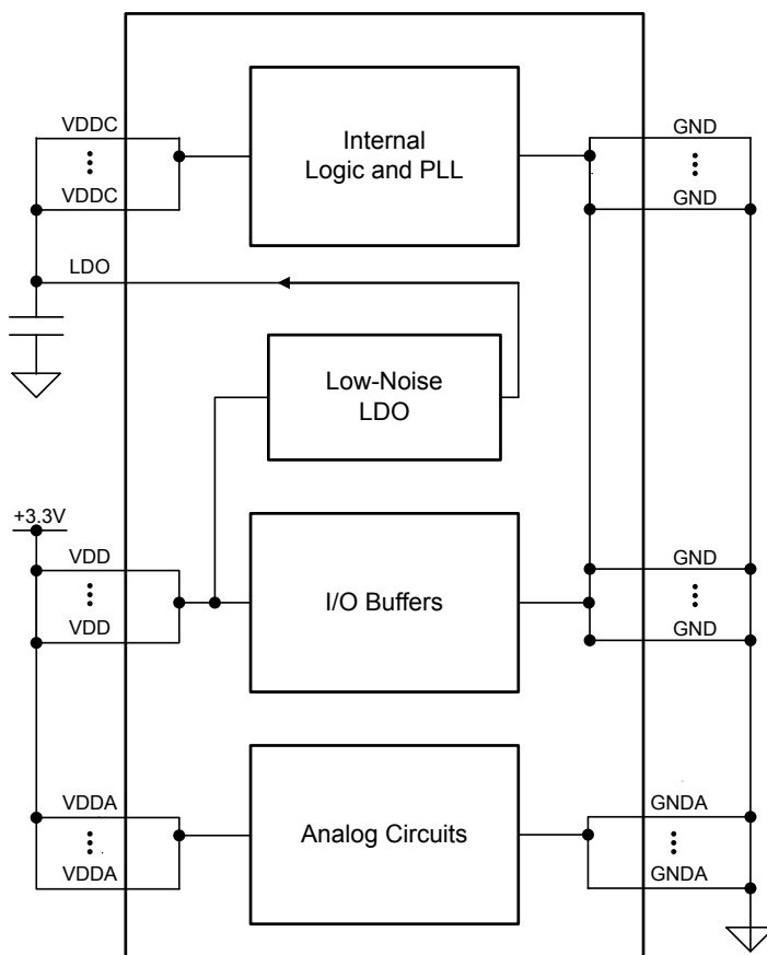
Figure 5-4. Power Architecture
