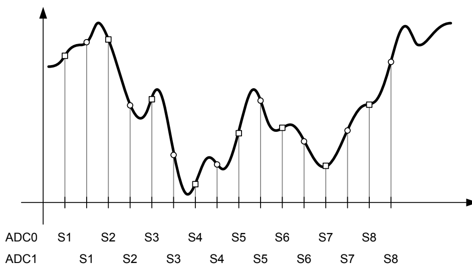
Figure 12-5. Skewed Sampling
