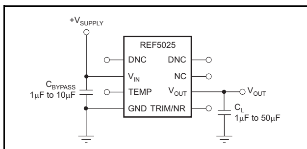
Figure 25. Basic Connections
