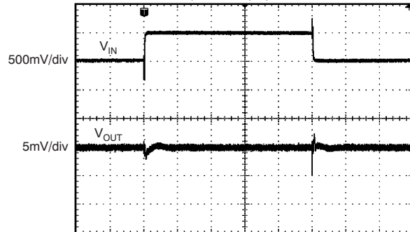
100 \mu\text{s}/\text{div} Figure 23.
