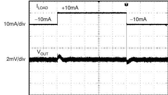
100 \mu\text{s}/\text{div} Figure 21.
