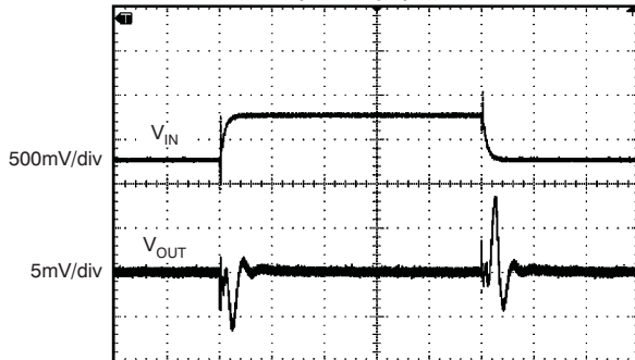
20 \mu\text{s}/\text{div} Figure 22.
