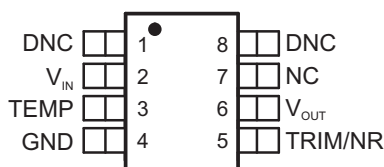
HKJ PACKAGE (TOP VIEW)
