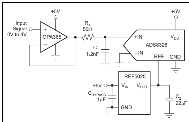
Figure 30. Basic Data Acquisition System
