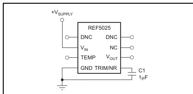
Figure 27. Noise Reduction Using TRIM/NR Pin
