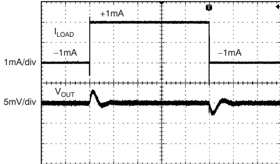
100 \mu\text{s}/\text{div} Figure 20.
