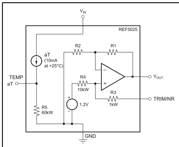
Figure 24. REF5025 Simplified Block Diagram
