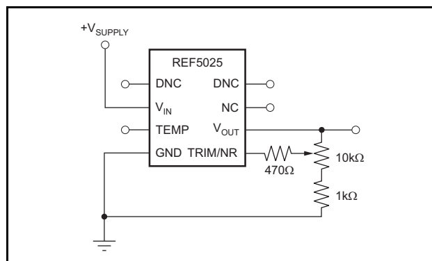
Figure 26. V_{OUT} Adjustment Using TRIM/NR Pin
