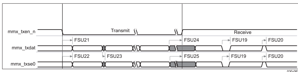
Figure 6-45. Low-/Full-Speed USB – Bidirectional Standard 3-pin Mode
