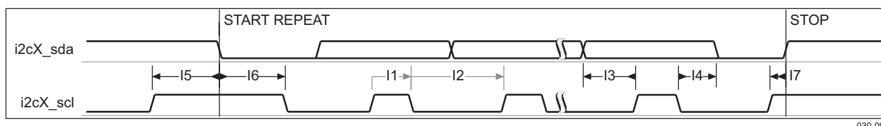
Figure 6-54. I 2 C – High-Speed Mode (1) (2) (3)
