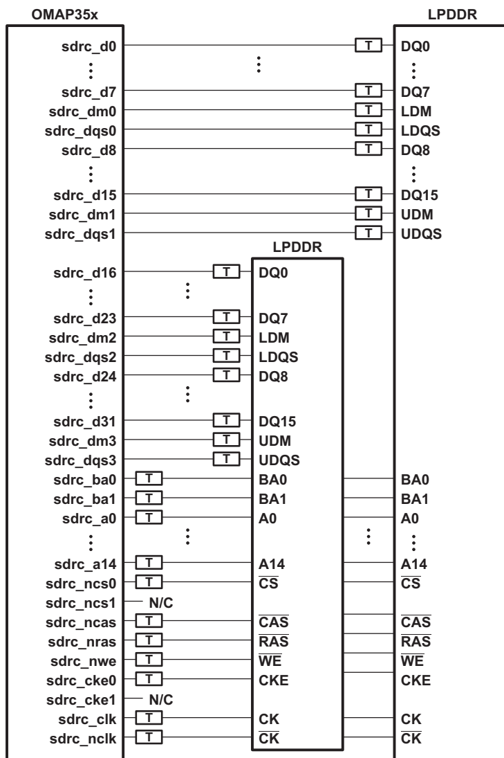
Figure 6-17. OMAP3503 LPDDR High Level Schematic (x16 memories)
