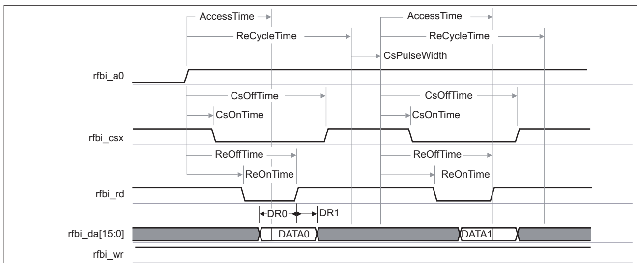
Figure 6-31. LCD Display in RFB Mode – Data Read Mode(1) (2)
