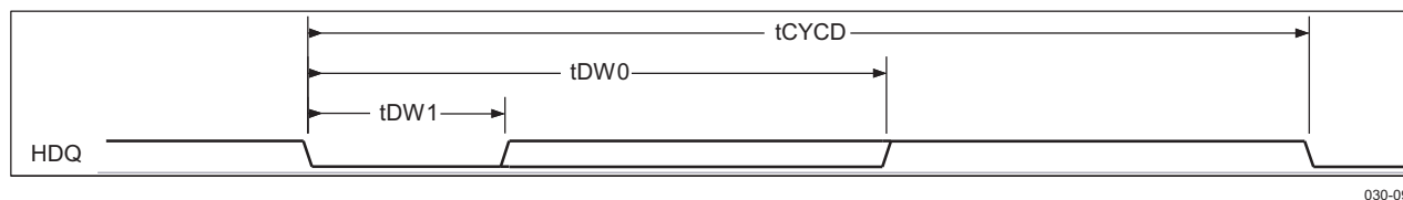
Figure 6-57. HDQ Write Bit Timing (Command/Address or Data)
