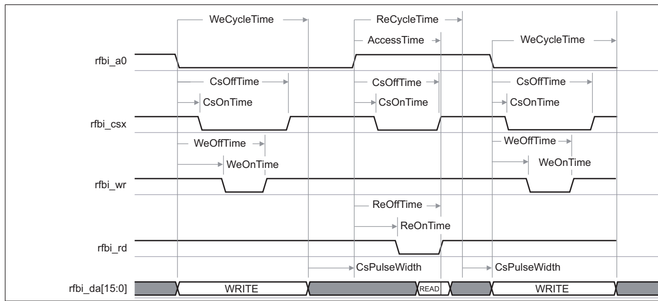
Figure 6-32. LCD Display in RFB Mode – Command / Data Write-to-Read and Read-to-Write Timing Modes(1) (2)
