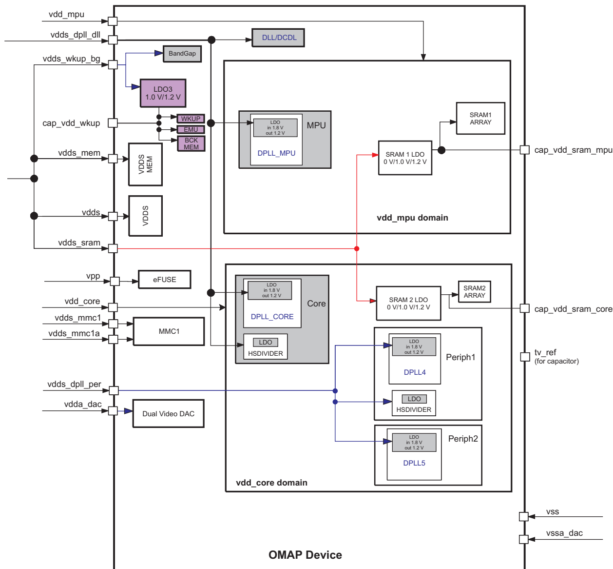
Figure 3-1. OMAP3503 Power Domains
