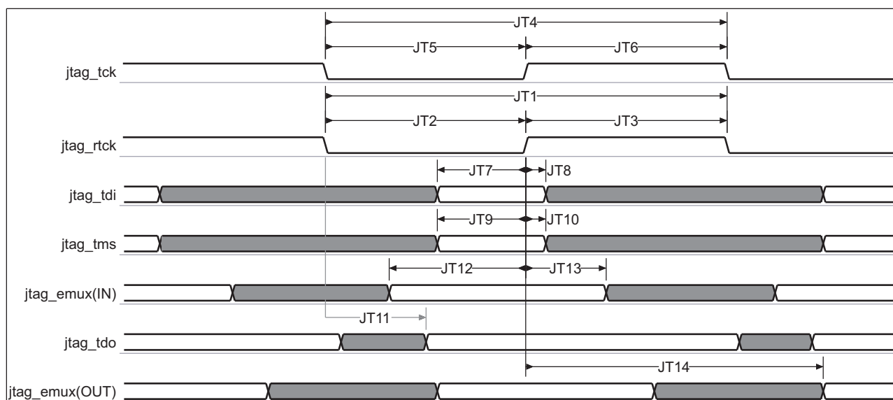
Figure 6-72. JTAG Interface Timing – Free Running Clock Mode
