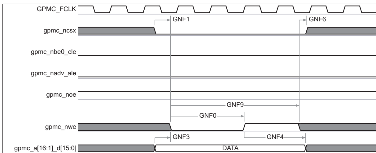
Figure 6-16. GPMC/NAND Flash – Data Write Cycle Timing
