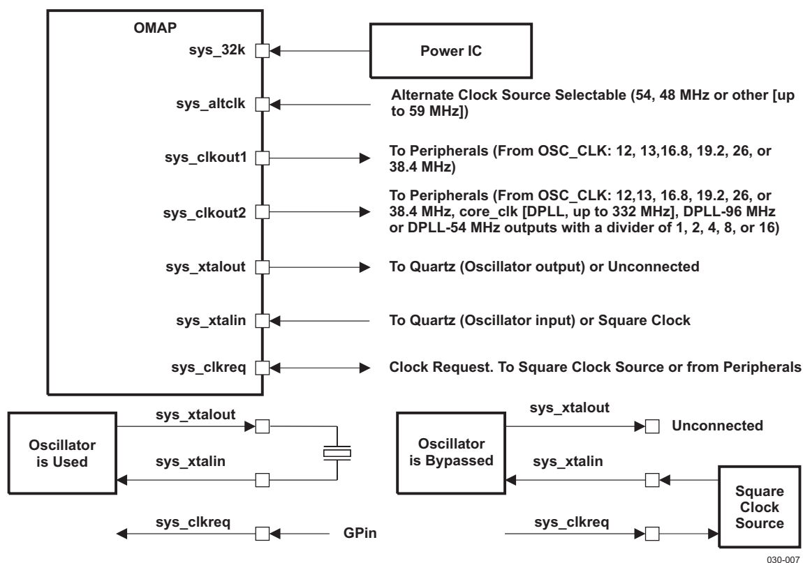
Figure 4-1. Clock Interface
