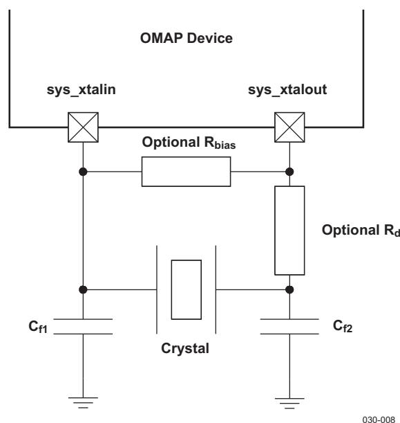
Figure 4-2. Crystal Implementation(1) (2) (3) (4)
