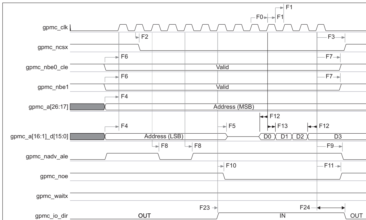
Figure 6-5. GPMC/Multiplexed NOR Flash – Synchronous Burst Read
