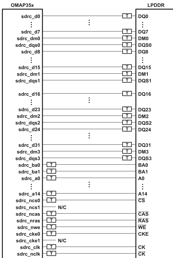
Figure 6-18. OMAP3503 LPDDR High Level Schematic (x32 memory)
