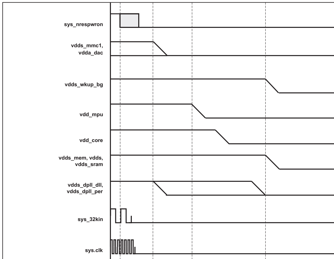
Figure 3-4. Power-down Sequence
