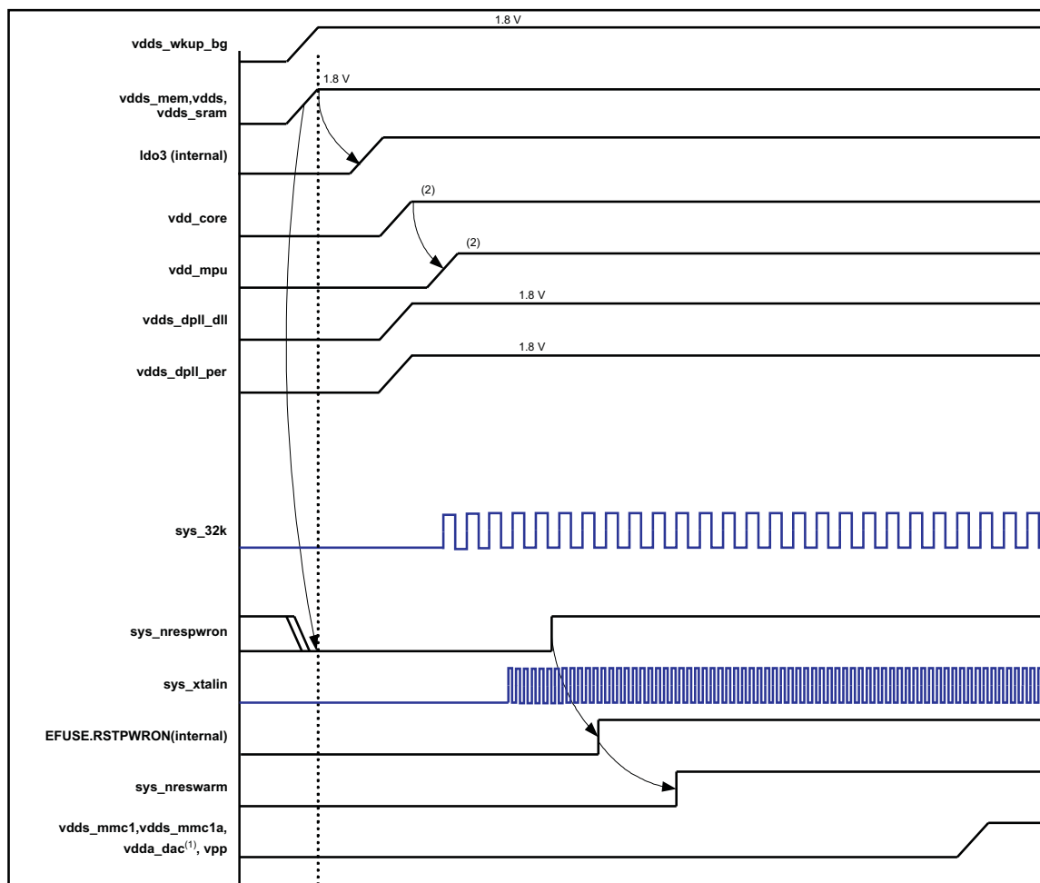
Figure 3-3. Power-up Sequence
