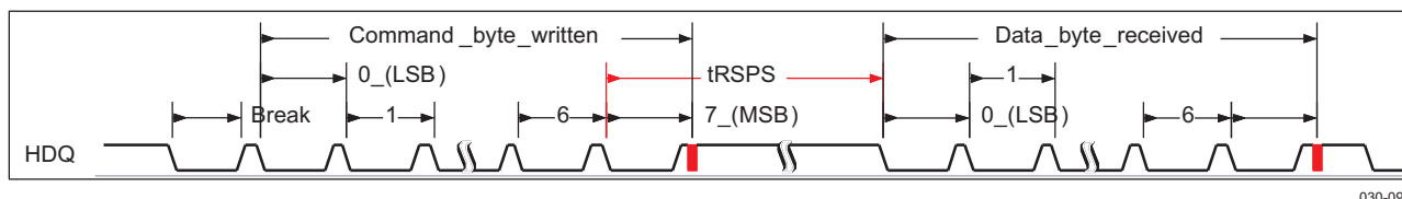
Figure 6-58. HDQ Communication Timing
