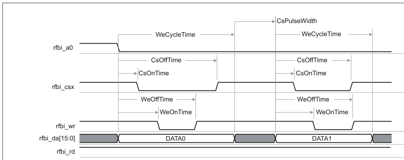
Figure 6-30. LCD Display in RFB Mode – Command / Data Write Mode(1) (2)
