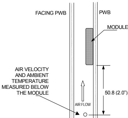
Note: Wind Tunnel Test Setup Figure Dimensions are in millimeters and (Inches)
