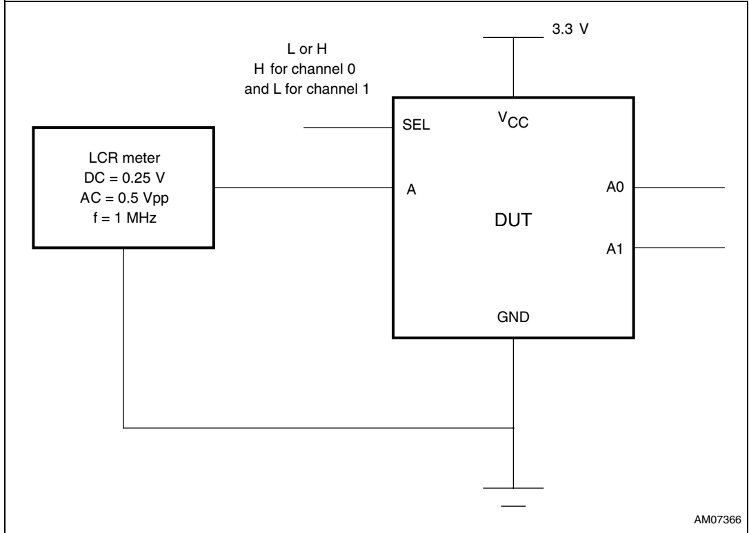
Figure 7. Test circuit for switch on capacitance ( C_{ON} )
