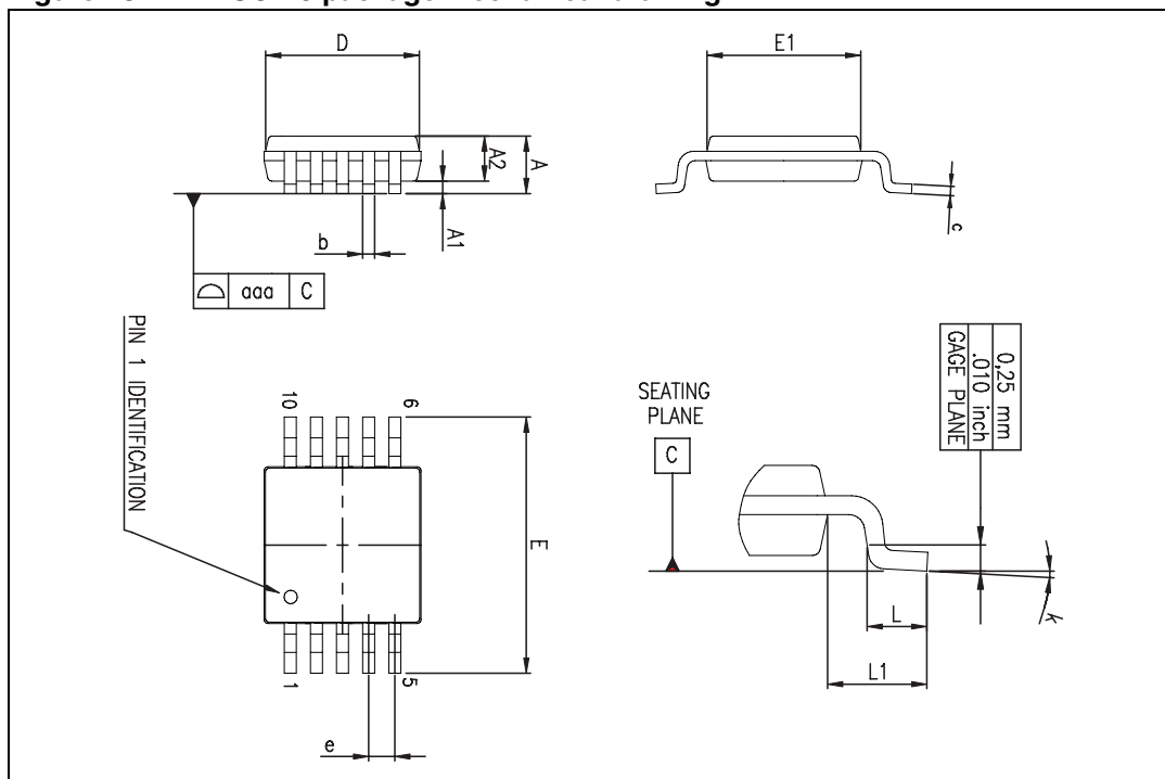
Figure 28. MiniSO-10 package mechanical drawing
