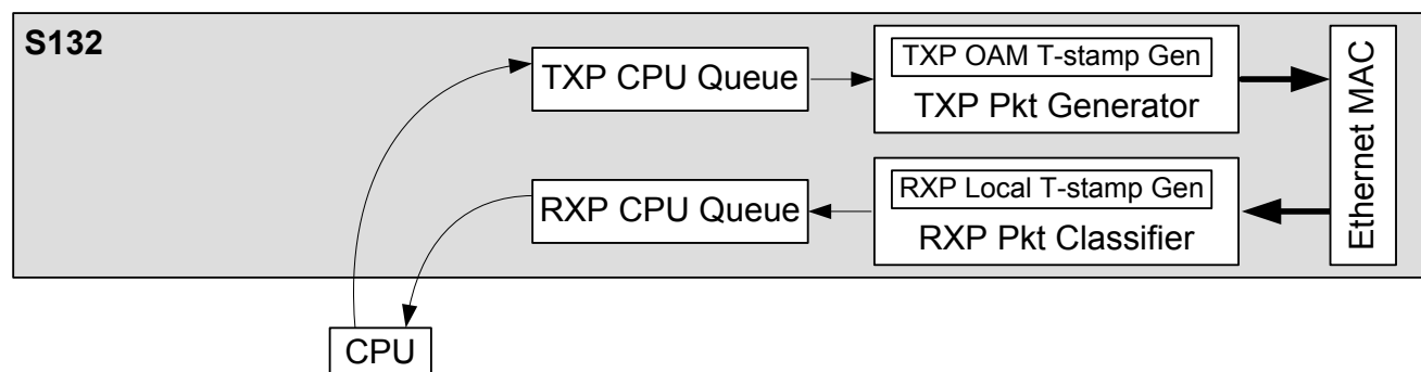
Figure 9-6. CPU Connections
