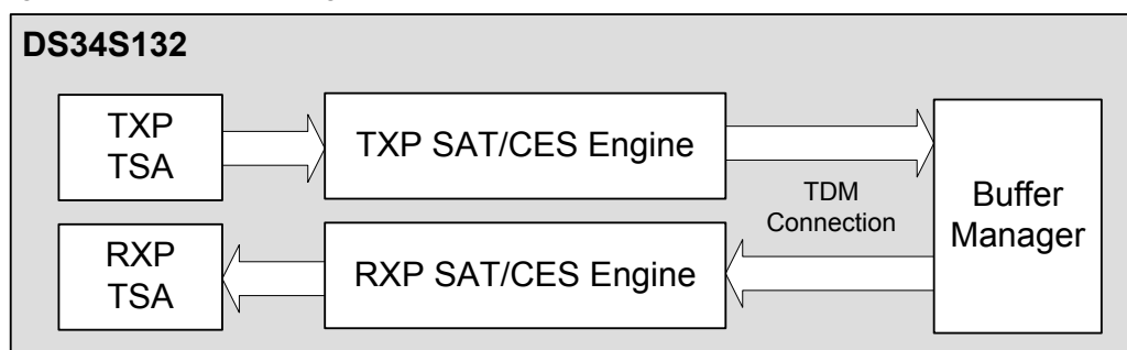
Figure 9-15. SAT/CES Engine Environment
