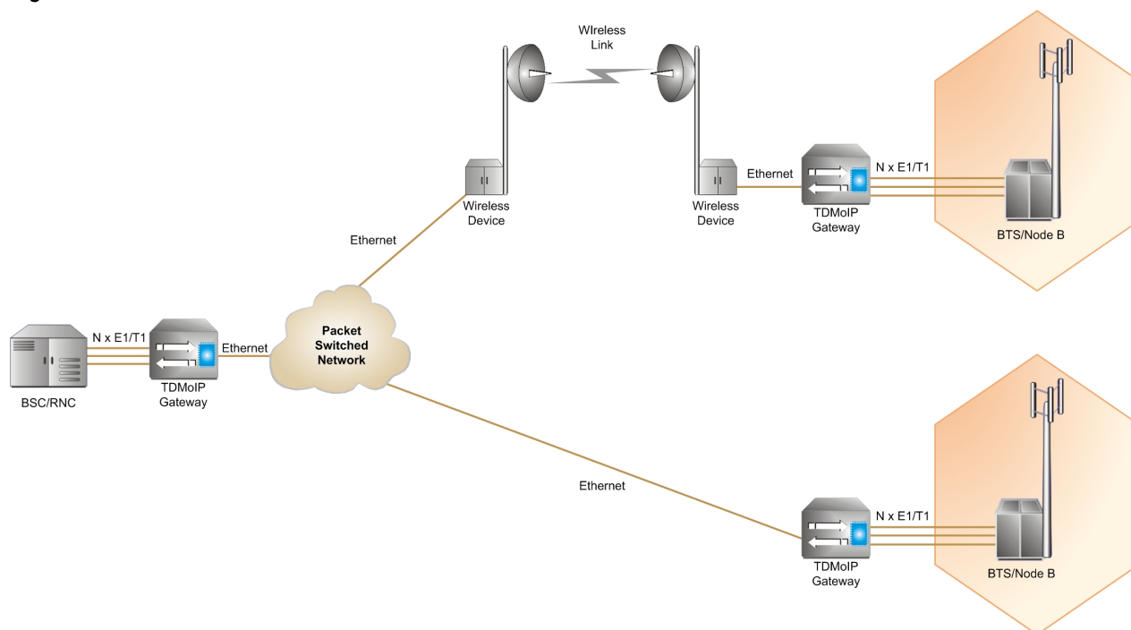
Figure 5-2. TDMoP in Cellular Backhaul
