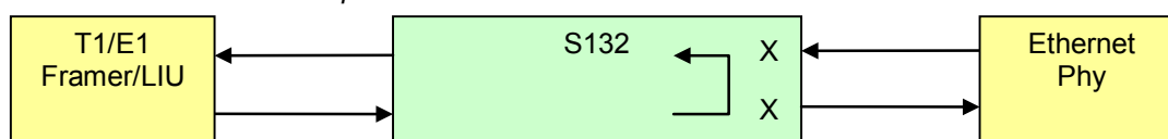
Figure 9-21. Ethernet Port Local Loopback
