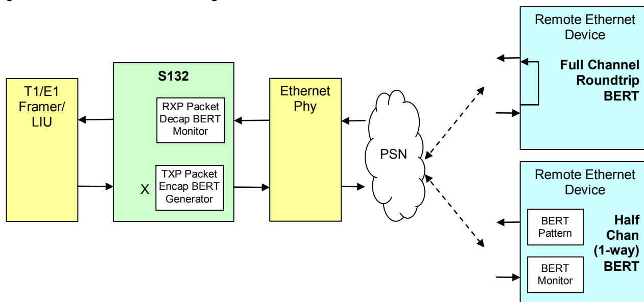
Figure 9-22. Ethernet Port BERT Diagram
