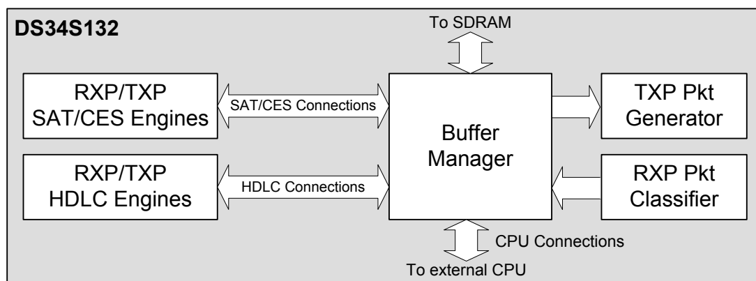
Figure 9-28. Buffer Manager Environment
