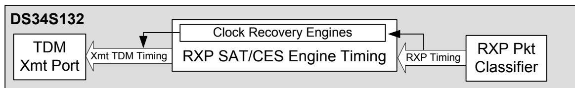
Figure 9-8. Clock Recovery Engine Environment
