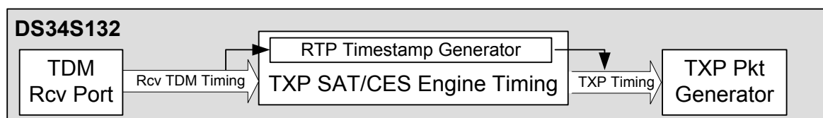
Figure 9-9. TXP PW-Timing Environment
