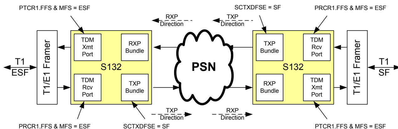
Figure 9-12. T1 ESF CAS to SF CAS Translation Example
