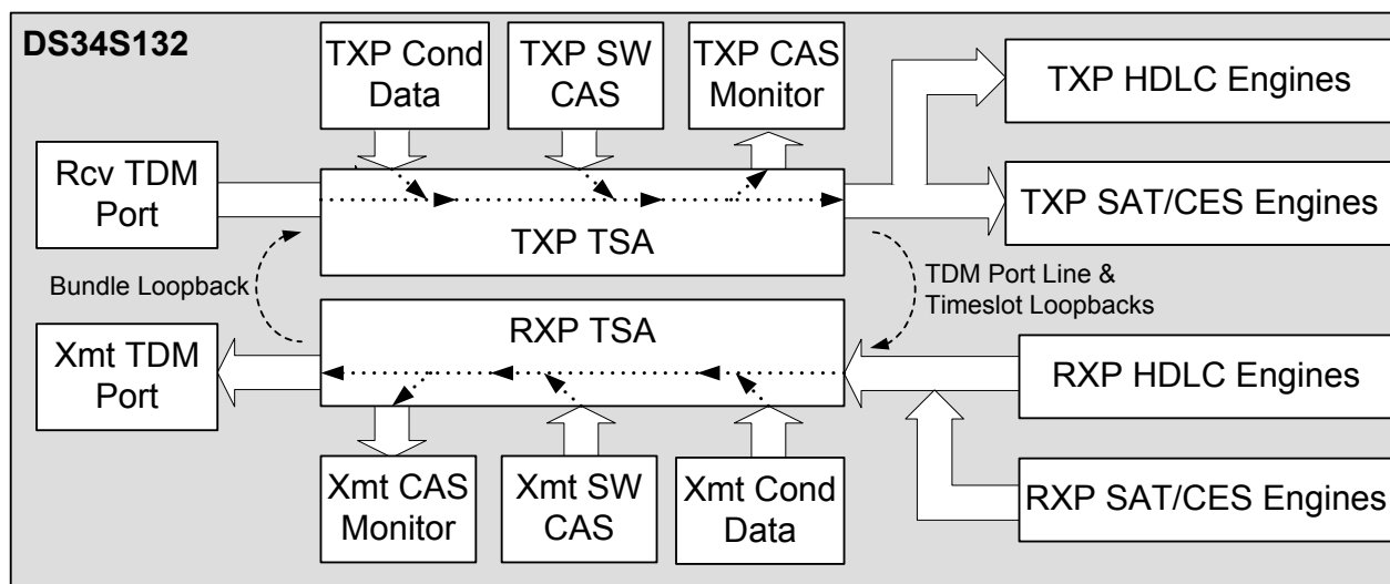
Figure 9-13. TSA Block Environment
