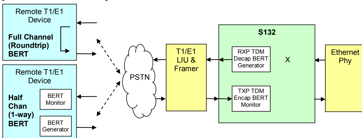
Figure 9-19. TDM Port BERT Diagram
