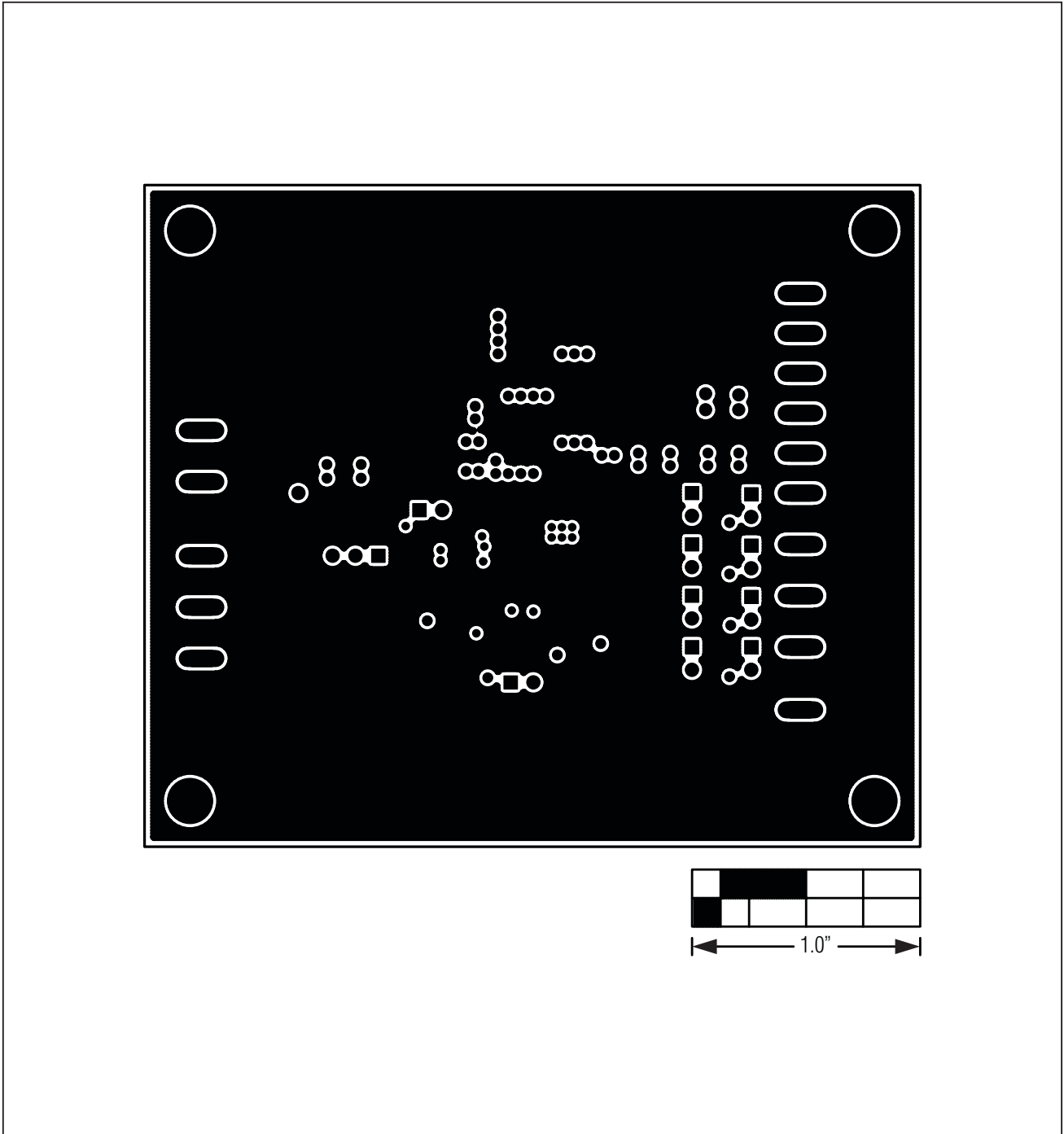
Figure 4. MAX16814 EV Kit PCB Layout—SGND Layer 2
