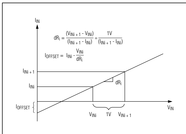
Figure 1. Effective Differential Input Resistance/Offset Current
