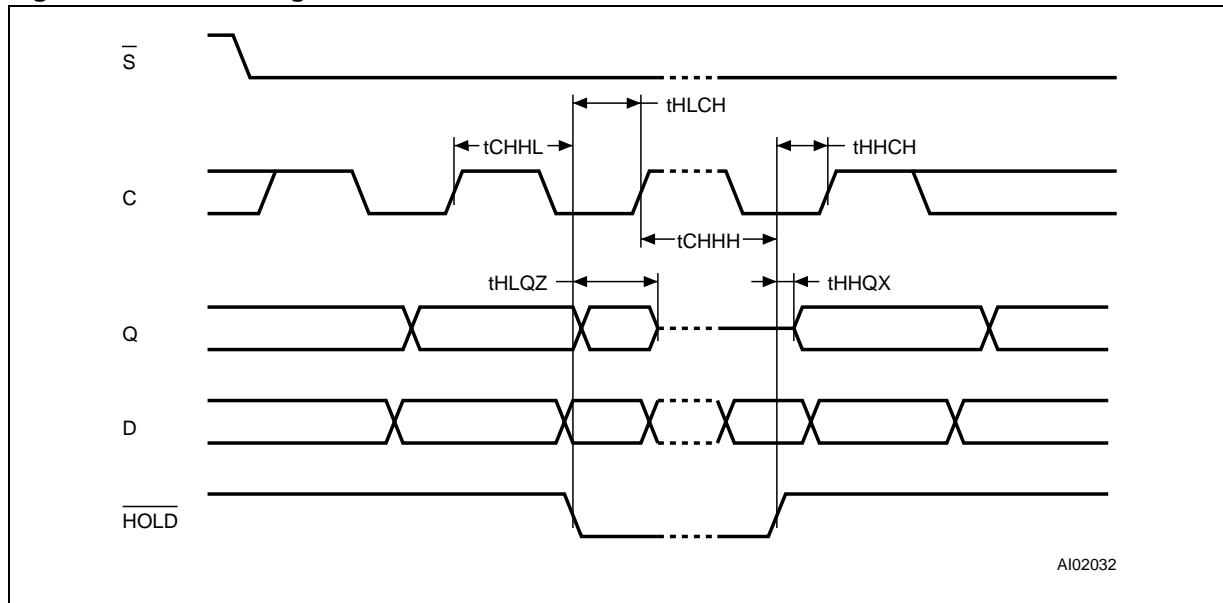
Figure 22. Hold timing
