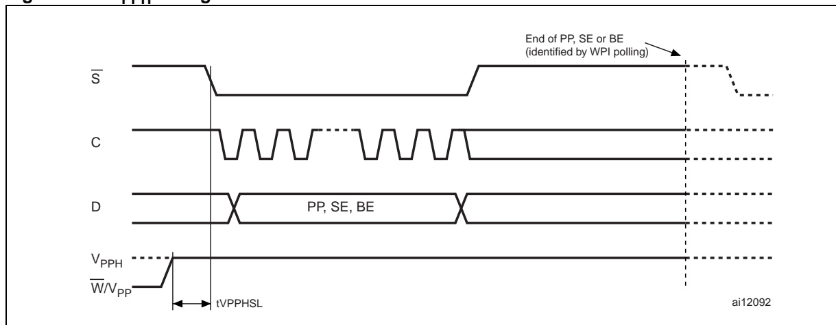
Figure 24. V_{PPH} timing
