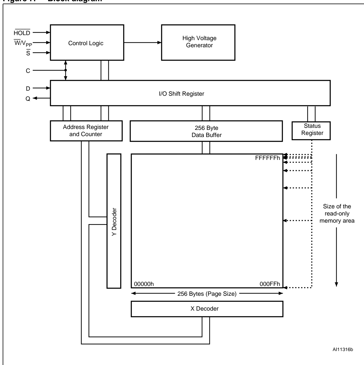
Figure 7. Block diagram
