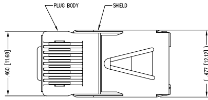
( SHOWN ASSEMBLED )
