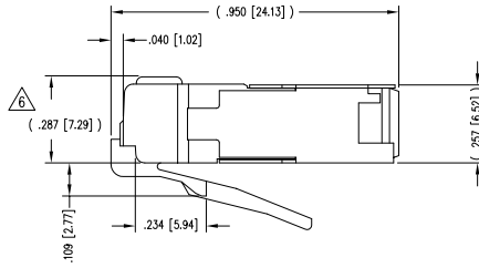
( SHOWN ASSEMBLED )
