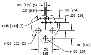
PC BOARD TOP VIEW
