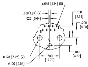
PC BOARD RECOMMENDED HOLE LAYOUT
