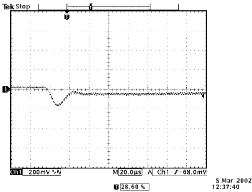
Vout=3.3V 50% to 100% load transients at 12.0V input and Ta=25° C
