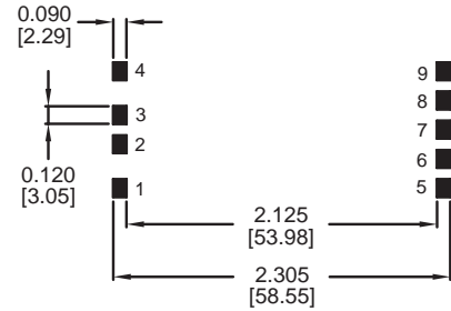
Recommended PCB Pad Layout
