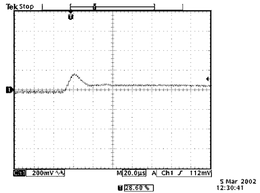
Vout=3.3V 100% to 50% load transients at 12.0V input and Ta=25° C
