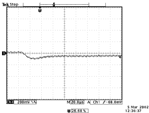
Vout=3.3V 50% to 100% load transients at 12.0V input and Ta=25° C
