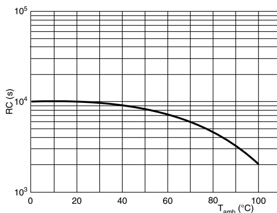
Insulation resistance (typical curve)
