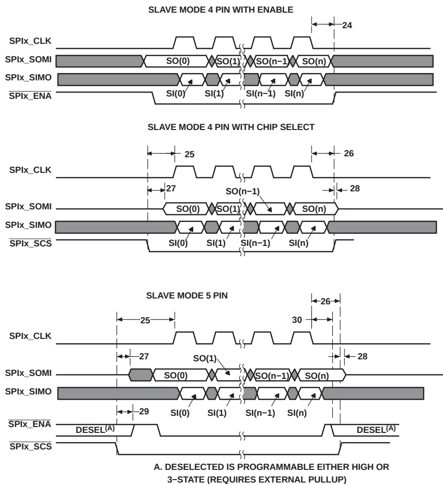
Figure 6-39. SPI Timings—Slave Mode (4-Pin and 5-Pin)
