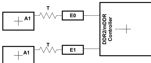
Figure 6-22. DQS and D Routing and Topology
