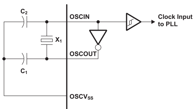
Figure 6-6. On-Chip Oscillator
