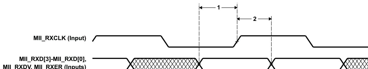
Figure 6-47. EMAC Receive Interface Timing
