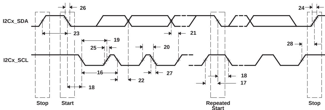
Figure 6-42. I2C Transmit Timings
