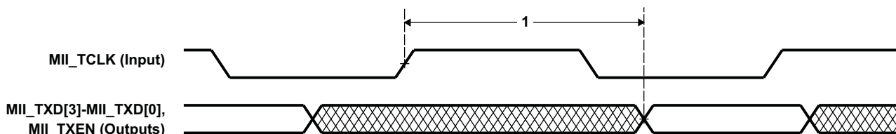
Figure 6-48. EMAC Transmit Interface Timing
