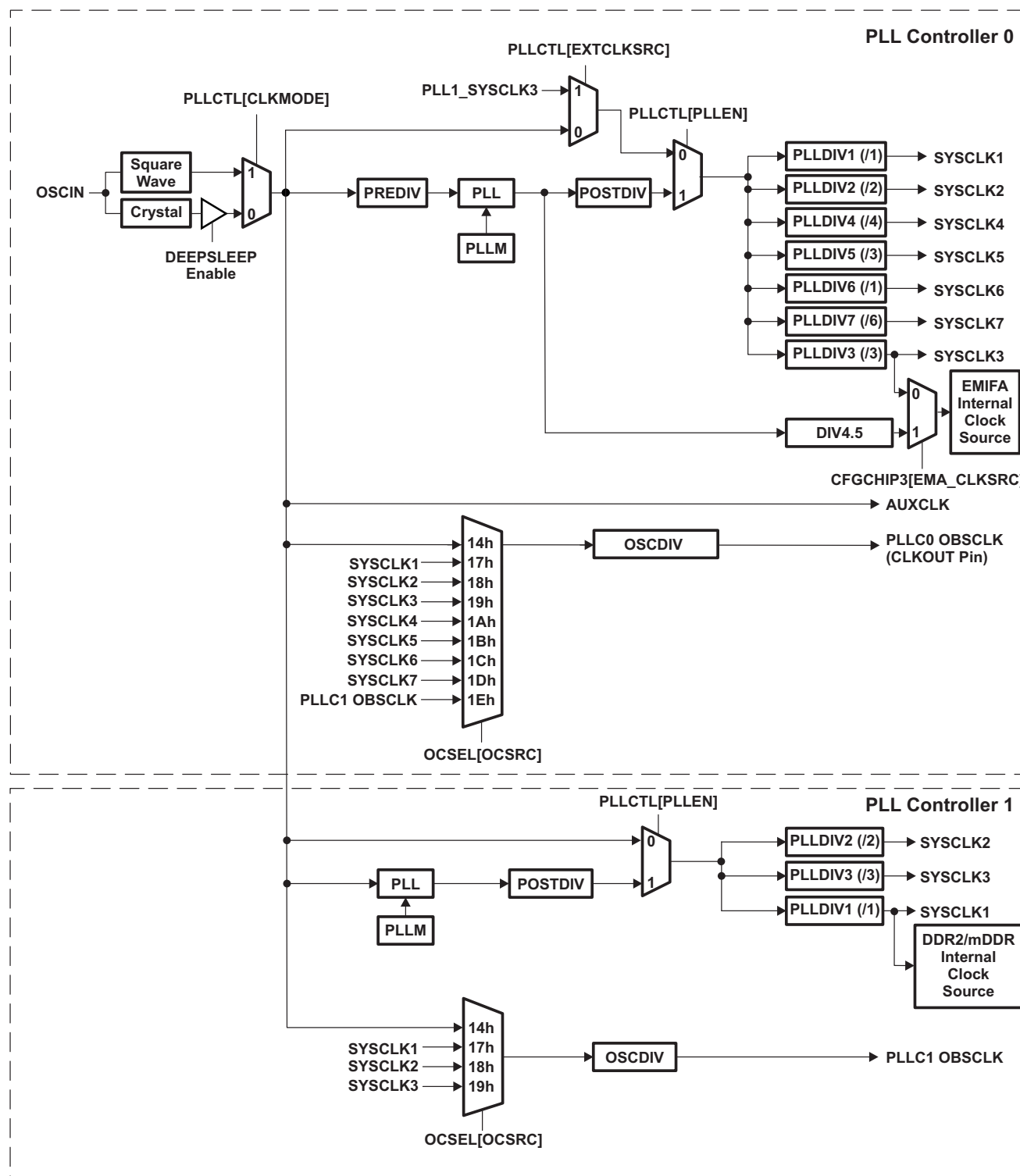
Figure 6-9. PLL Topology
