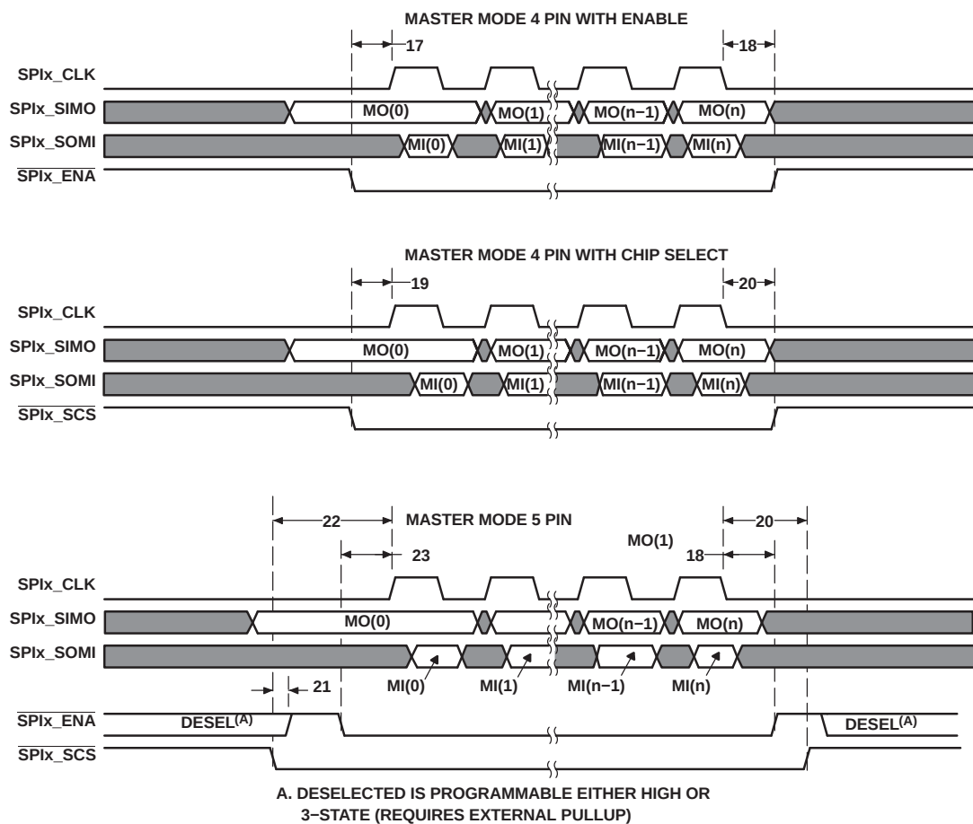
Figure 6-38. SPI Timings—Master Mode (4-Pin and 5-Pin)
