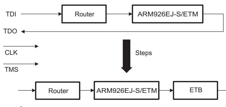
Figure 6-87. Adding ETB to the scan chain
