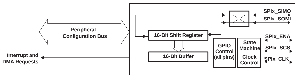
Figure 6-34. Block Diagram of SPI Module
