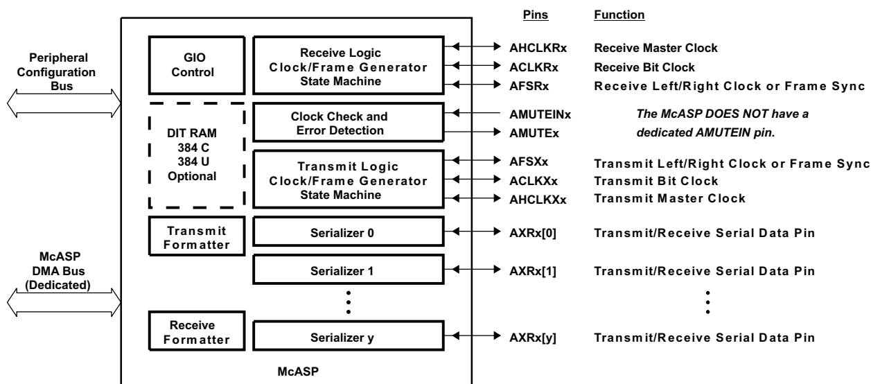
Figure 6-29. McASP Block Diagram
