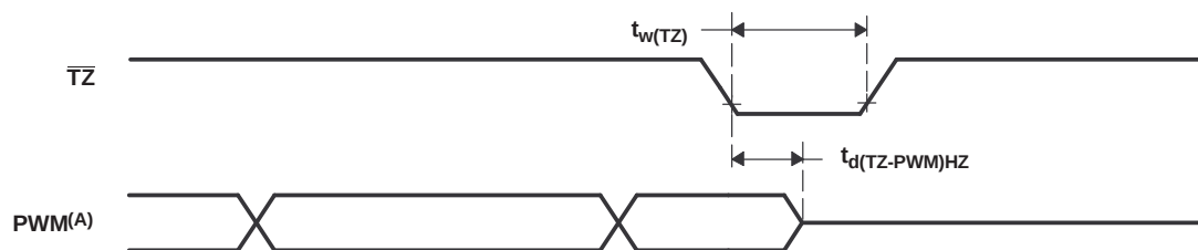
Figure 6-79. PWM Hi-Z Characteristics
