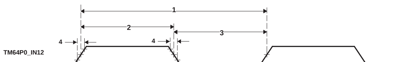
Figure 6-80. Timer Timing
