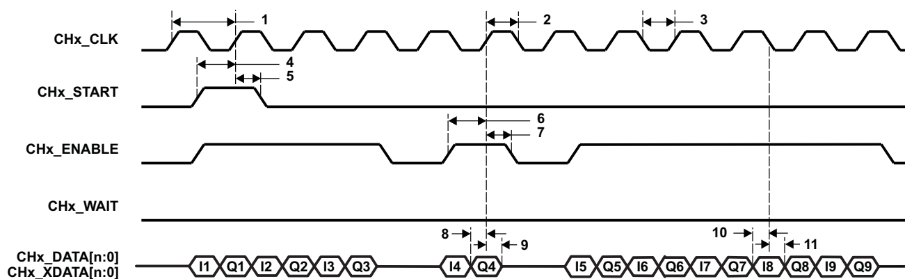
Figure 6-70. uPP Double Data Rate (DDR) Receive Timing
