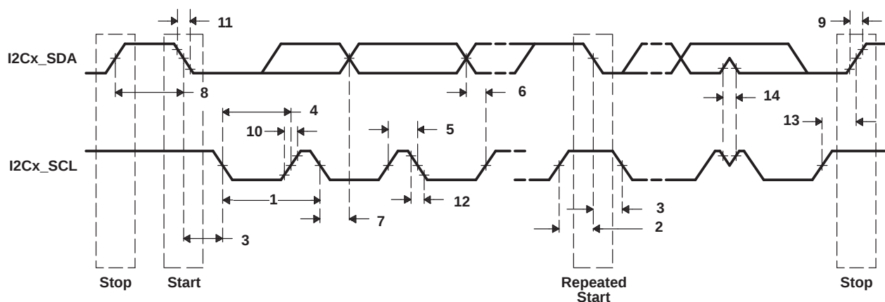
Figure 6-41. I2C Receive Timings
