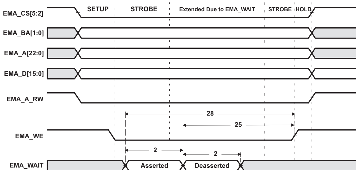
Figure 6-15. EMA_WAIT Write Timing Requirements
