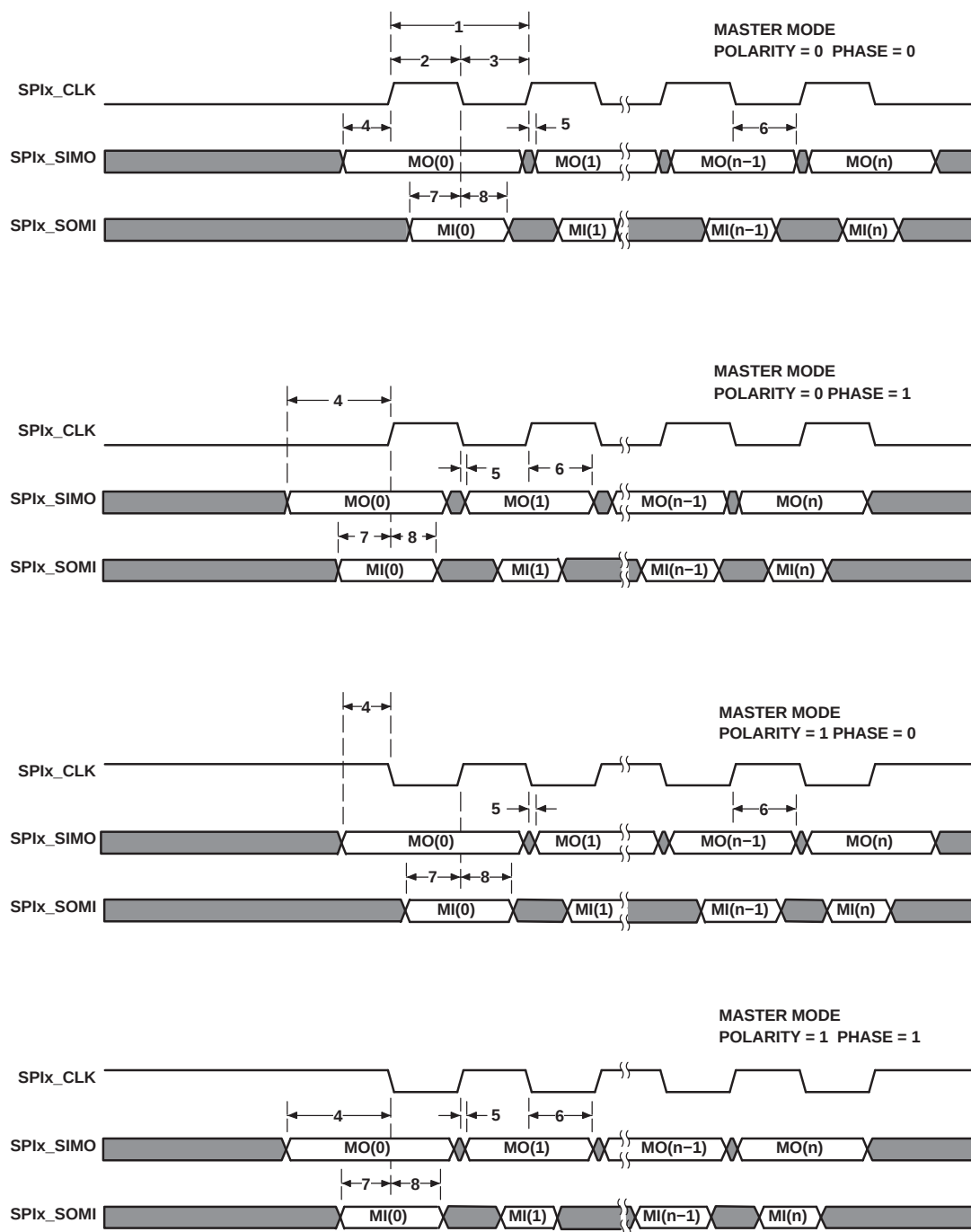
Figure 6-36. SPI Timings—Master Mode
