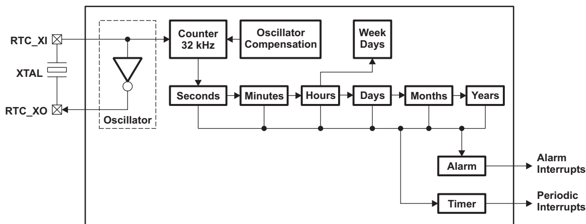
Figure 6-82. Real-Time Clock Block Diagram
