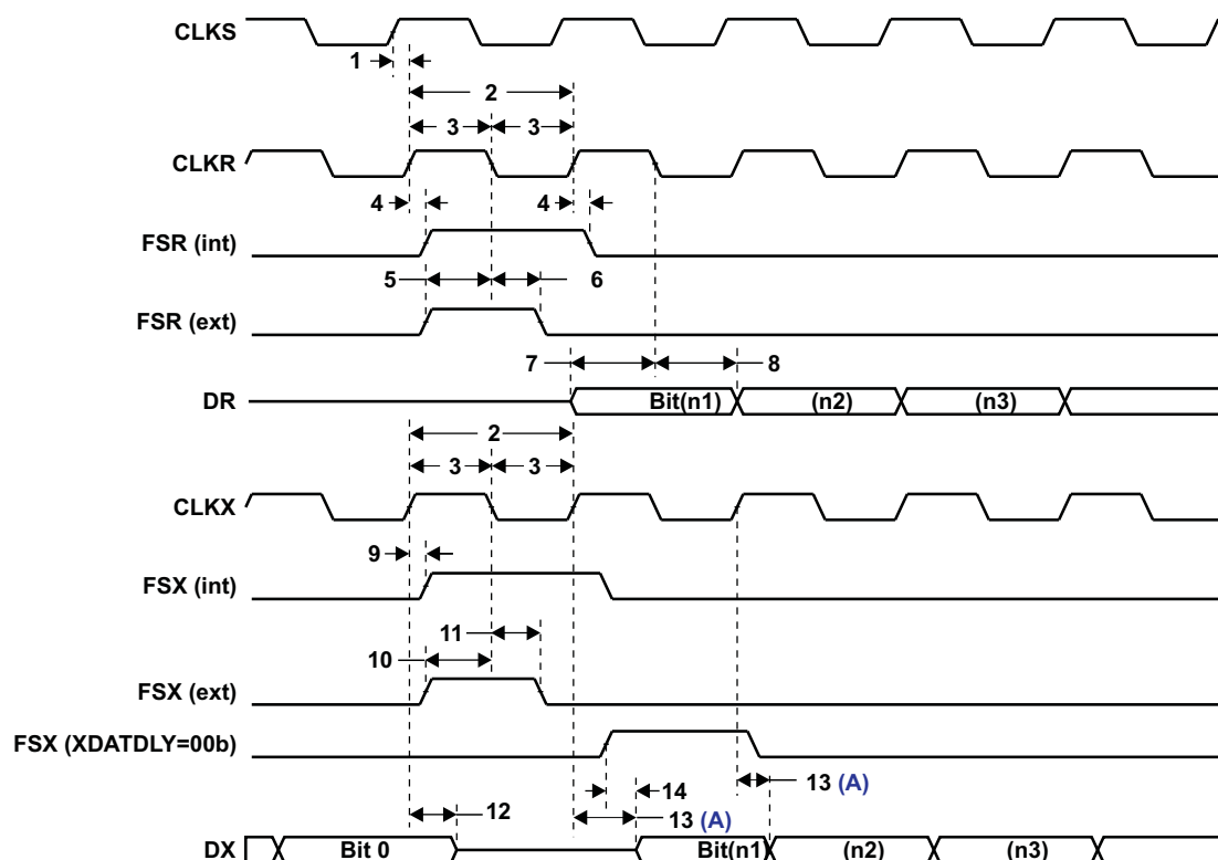
Figure 6-32. McBSP Timing
