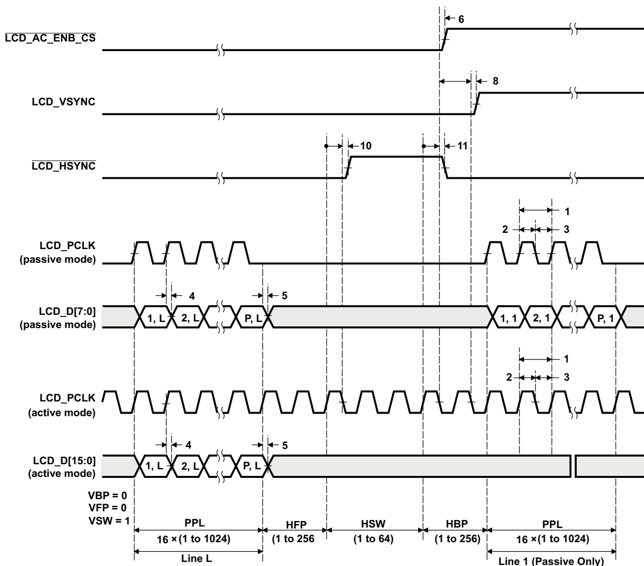
Figure 6-63. LCD Raster-Mode Control Signal Activation
