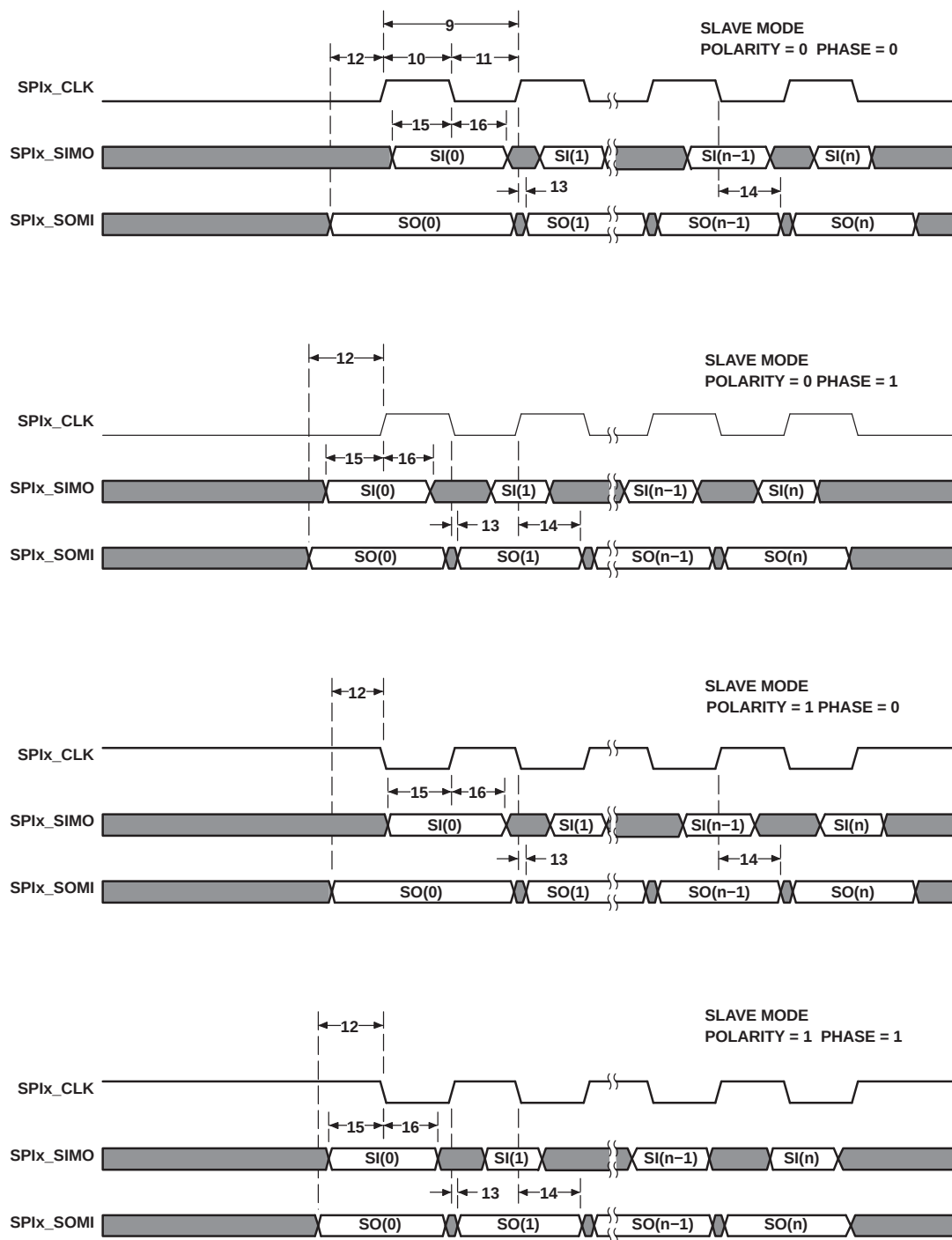
Figure 6-37. SPI Timings—Slave Mode
