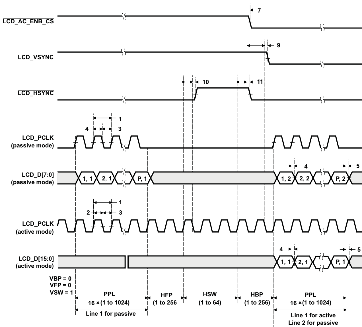
Figure 6-64. LCD Raster-Mode Control Signal Deactivation
