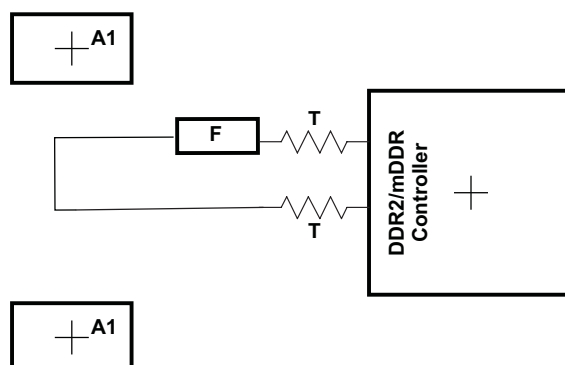
Figure 6-23. DQGATE Routing
