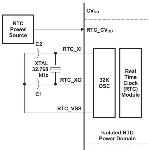
Figure 6-83. Clock Source
