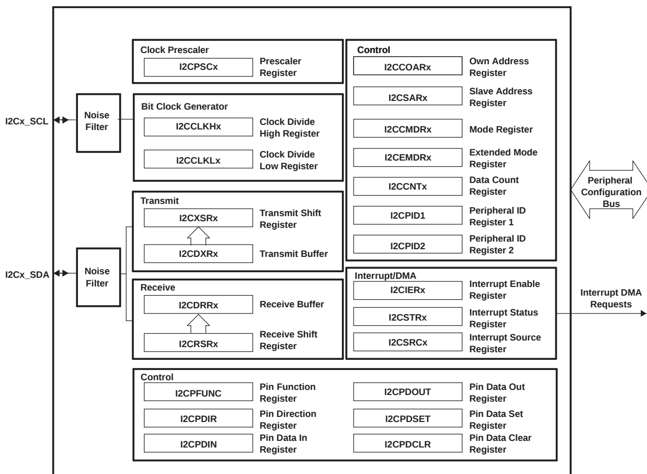
Figure 6-40. I2C Module Block Diagram
