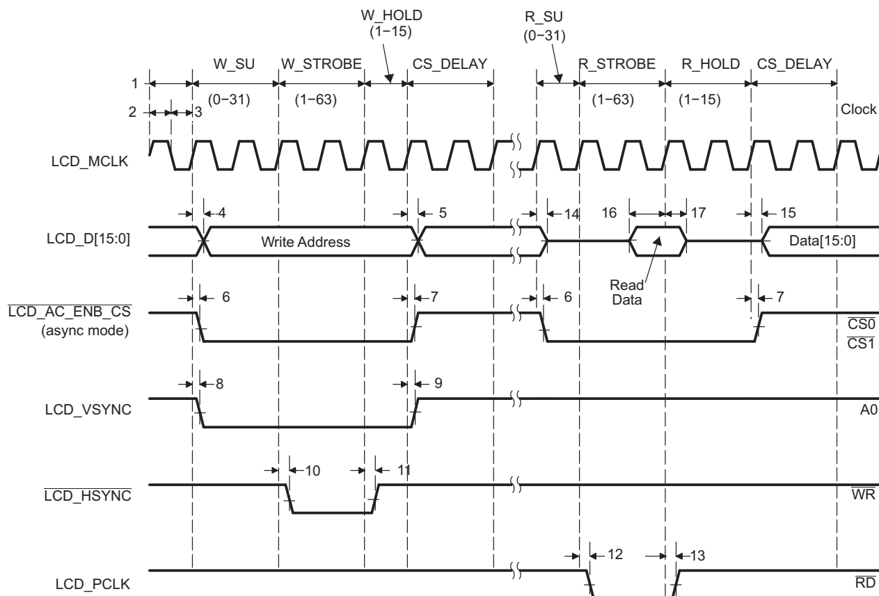
Figure 6-58. Micro-Interface Graphic Display 8080 Read
