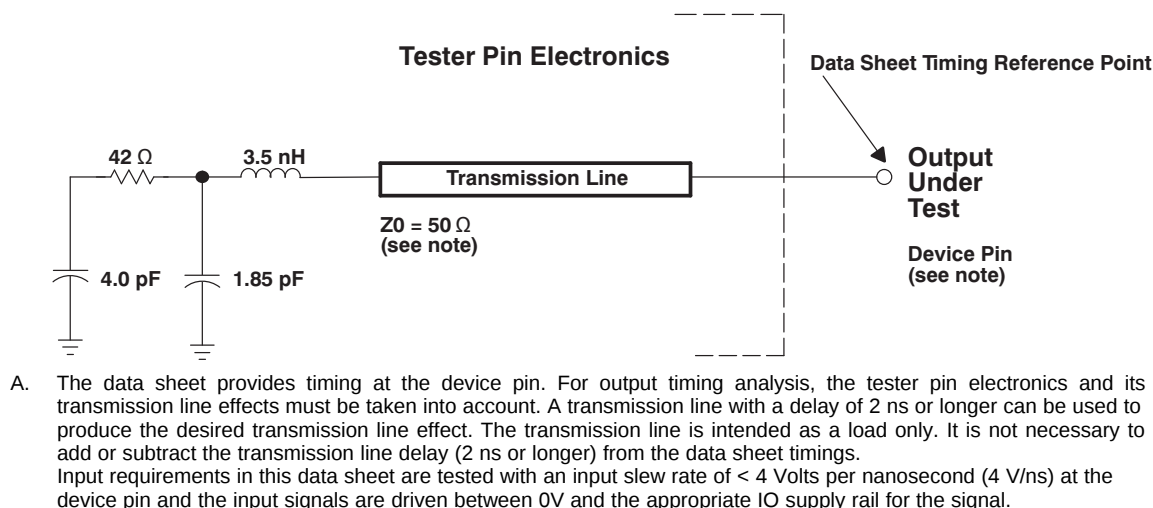
Figure 6-1. Test Load Circuit for AC Timing Measurements
