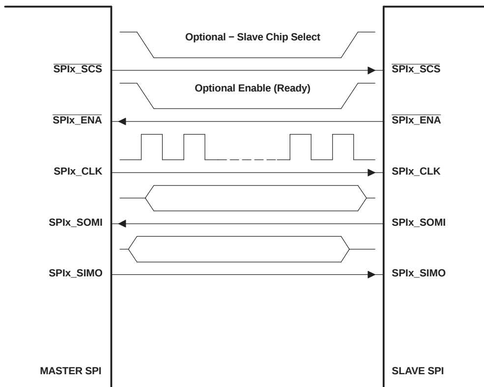
Figure 6-35. Illustration of SPI Master-to-SPI Slave Connection
