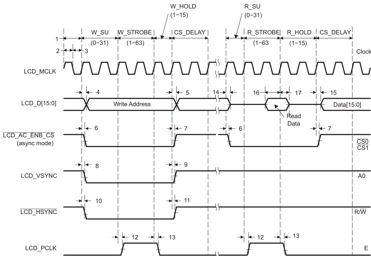
Figure 6-55. Micro-Interface Graphic Display 6800 Read
