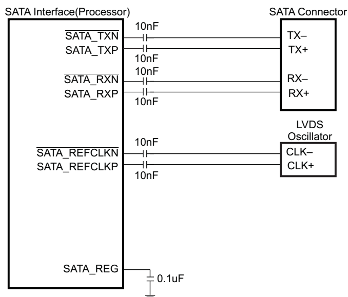
Figure 6-28. SATA Interface High Level Schematic
