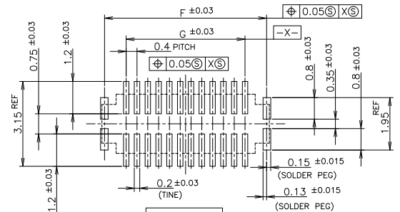
REFERENCE PCB LAYOUT SCALE 10:1
