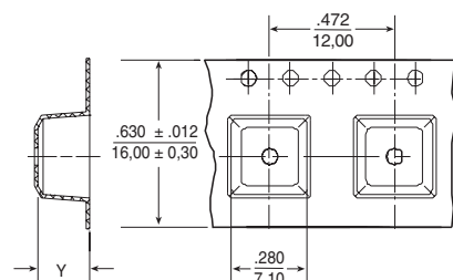
TAPE & REEL LAYOUT
