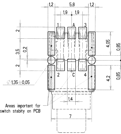
RECOMMENDED PCB LAYOUT ( WITH HOLES ) TOP VIEW
