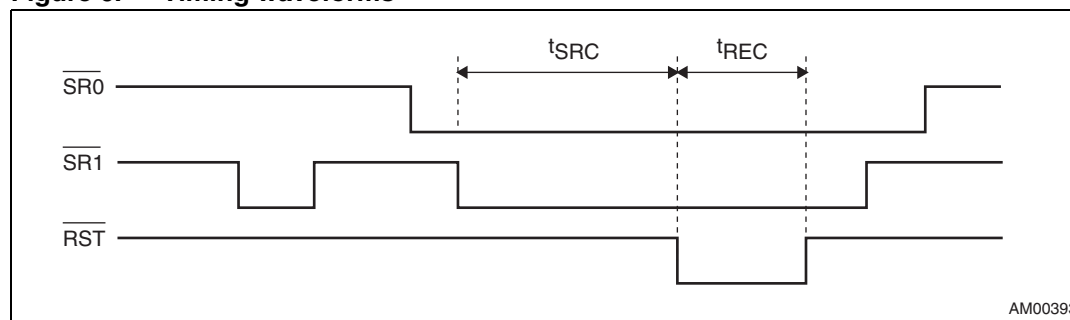
Figure 6. Timing waveforms
