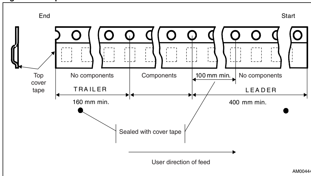
Figure 16. Tape trailer/leader
