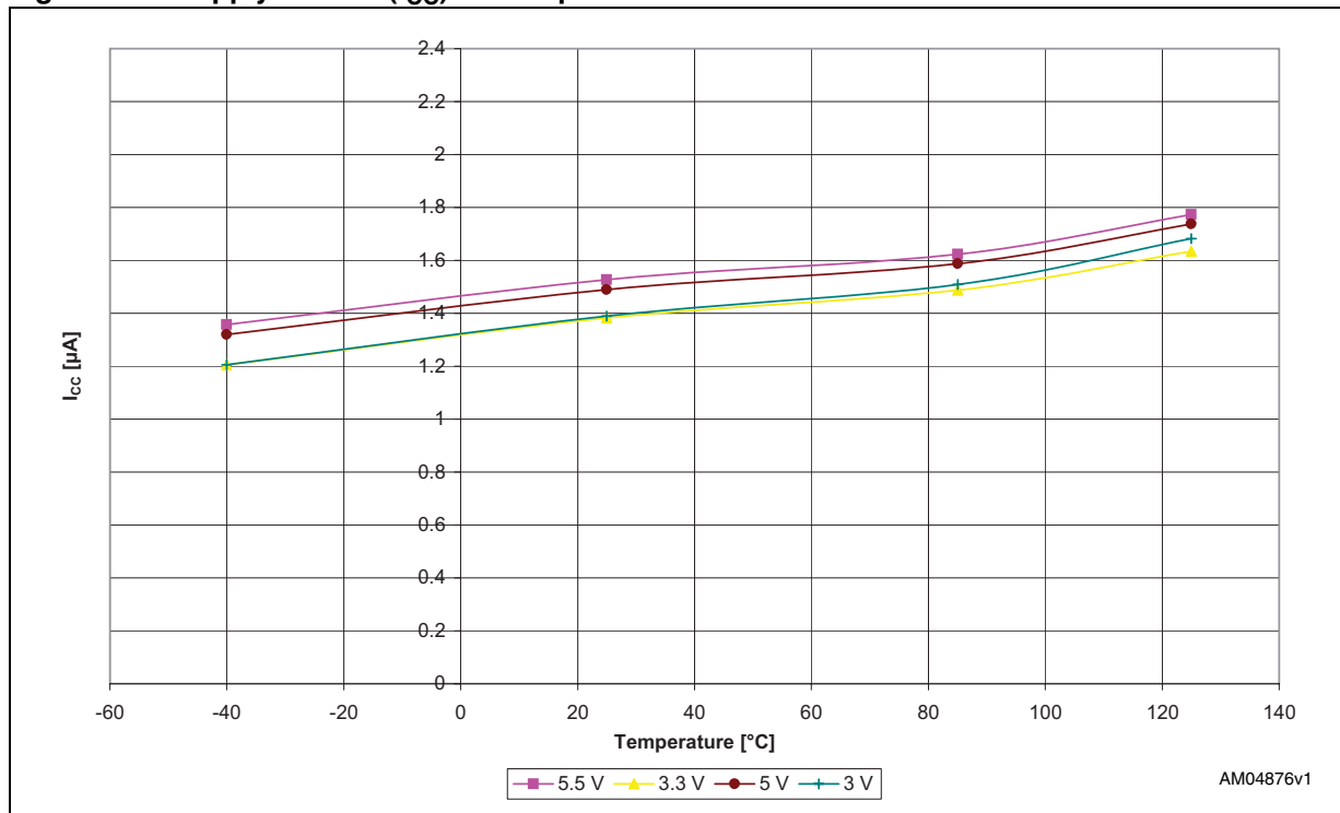
Figure 7. Supply current ( I_{CC} ) vs. temperature
