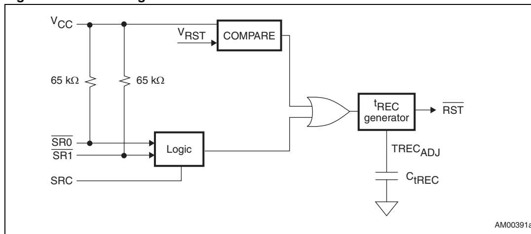
Figure 3. Block diagram
