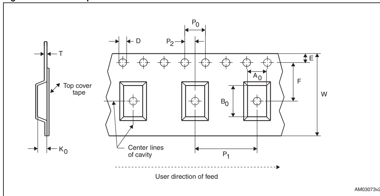
Figure 14. Carrier tape
