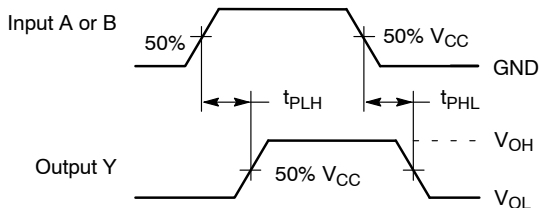
Figure 3. Switching Waveforms
