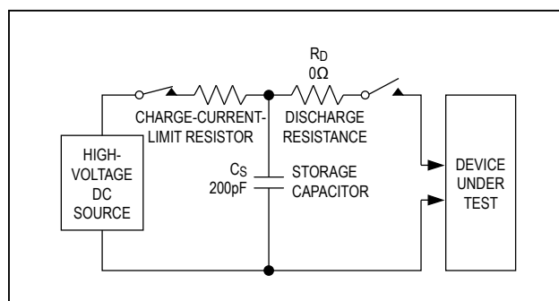
Figure 2. Machine Model ESD Test Circuit
