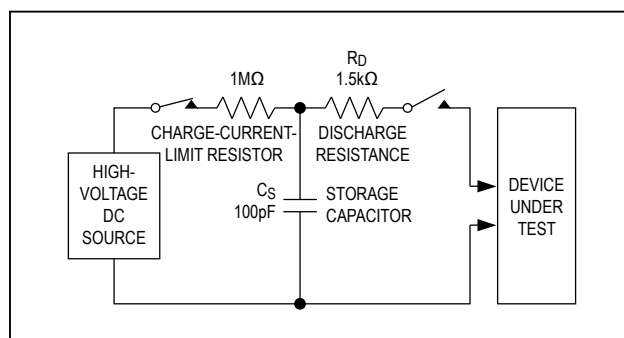
Figure 1. Human Body ESD Test Circuit
