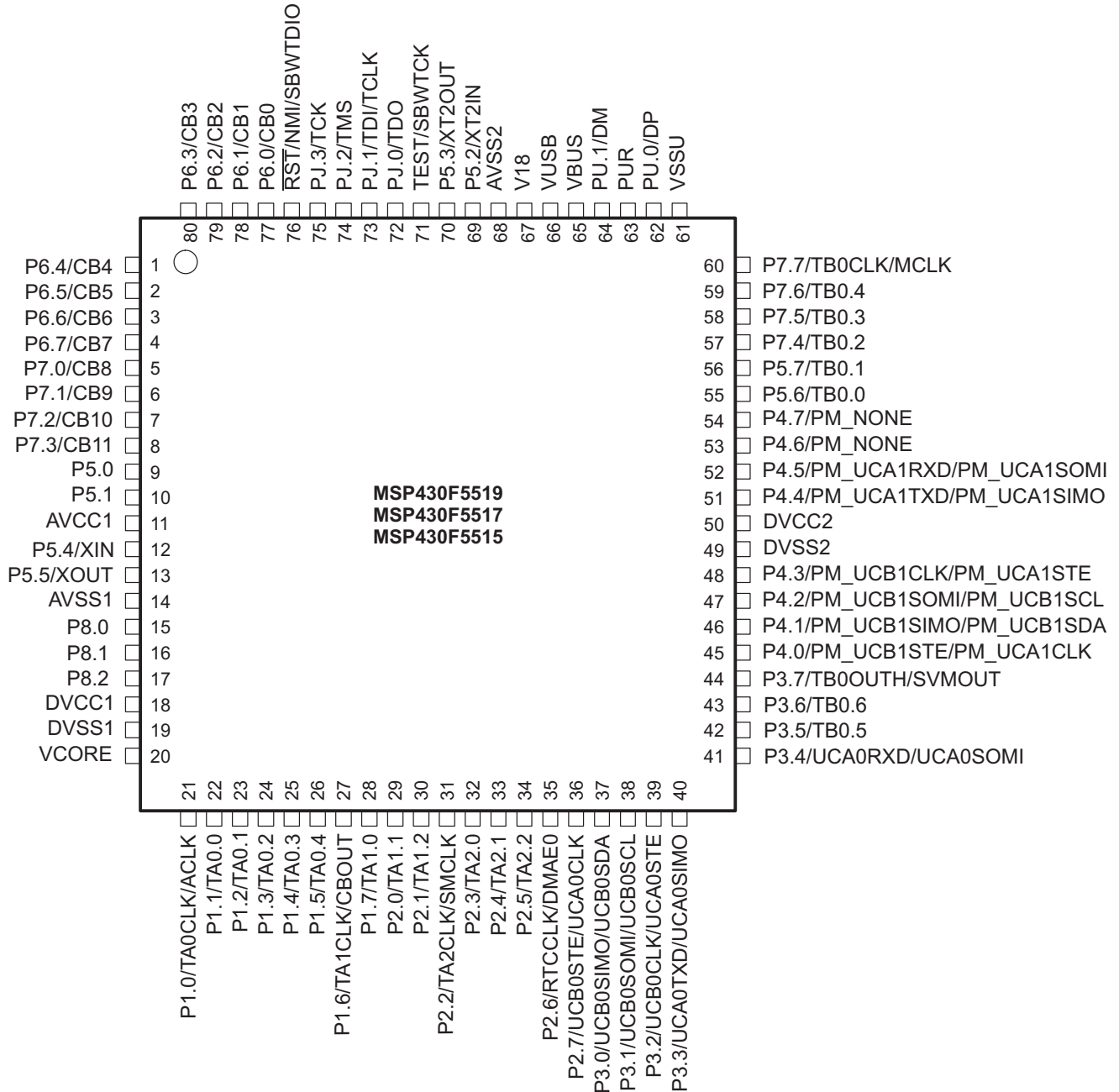
Figure 4-3. Pin Designation – MSP430F5519IPN, MSP430F5517IPN, MSP430F5515IPN (Top View)
