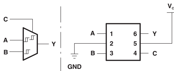
Figure 1. 2-to-1 Data Selector/Multiplexer
