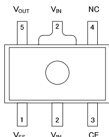
SOT-89-5 (TOP VIEW)
