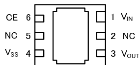
USP-6B (BOTTOM VIEW)
