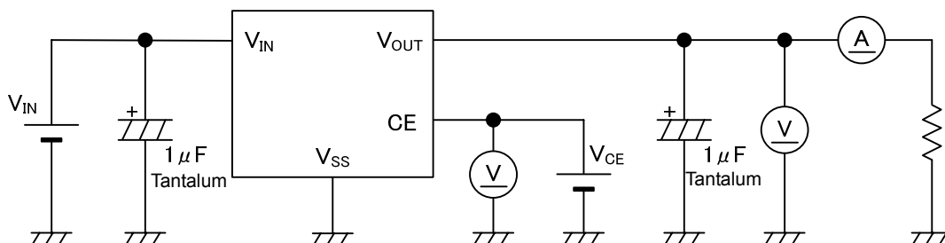
Circuit 1
