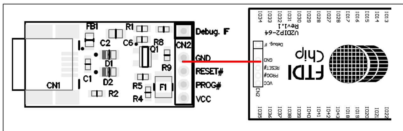
Figure 3.2 Example Connection of Debug Module Connection to V2DIP2-64
