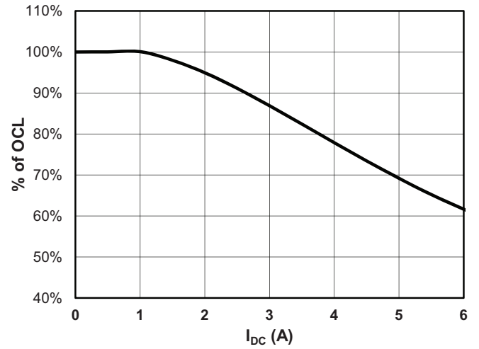
HCM0703-330-R
