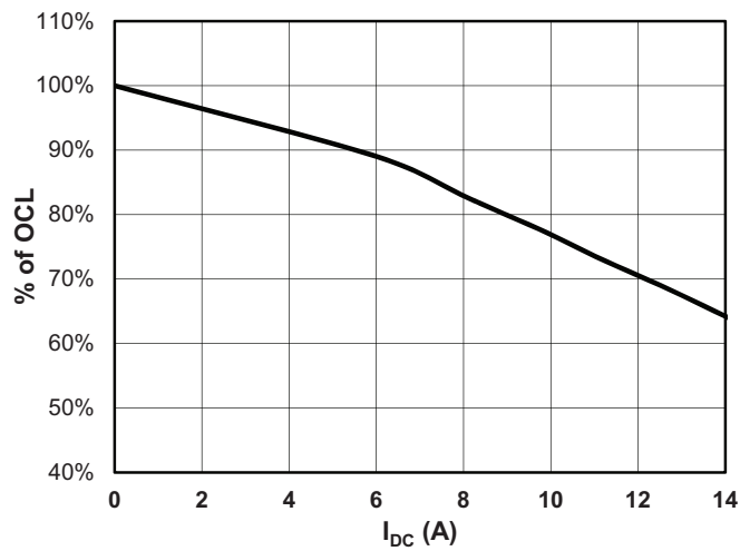
HCM0703-100-R
