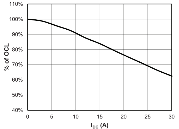
HCM0703-2R2-R
