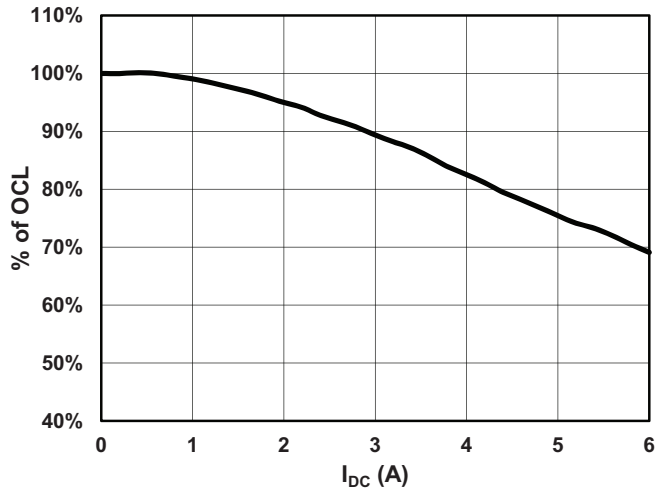
HCM0703-220-R
