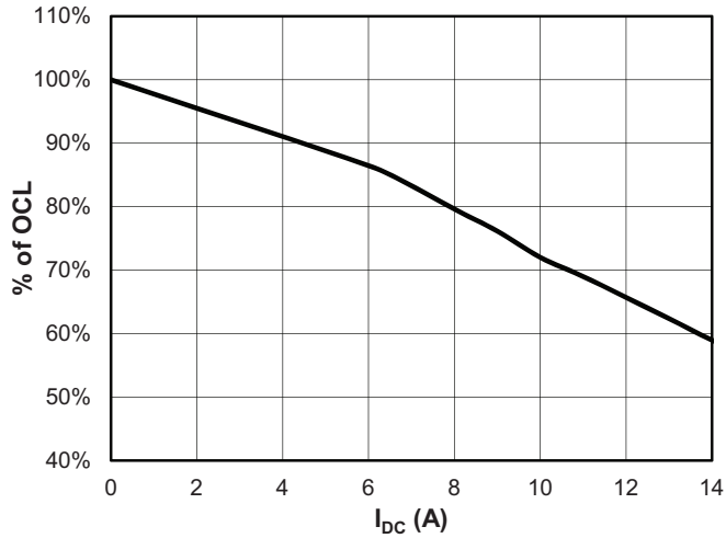
HCM0703-100-R
