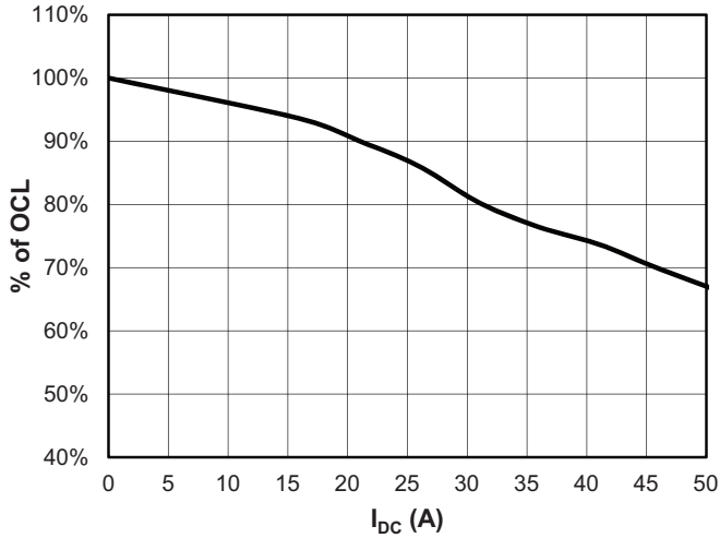
HCM0703-R47-R
