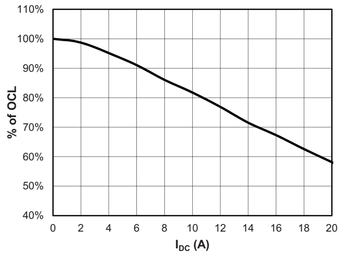
HCM0703-4R7-R
