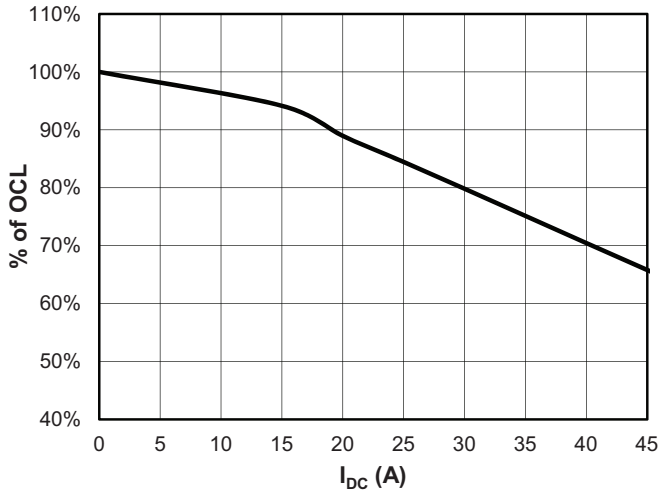
HCM0703-R82-R
