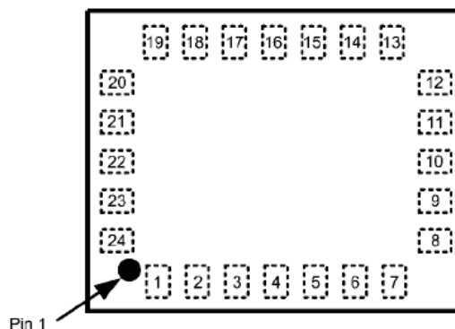
RHf PACKAGE MARKING - TOP VIEW
