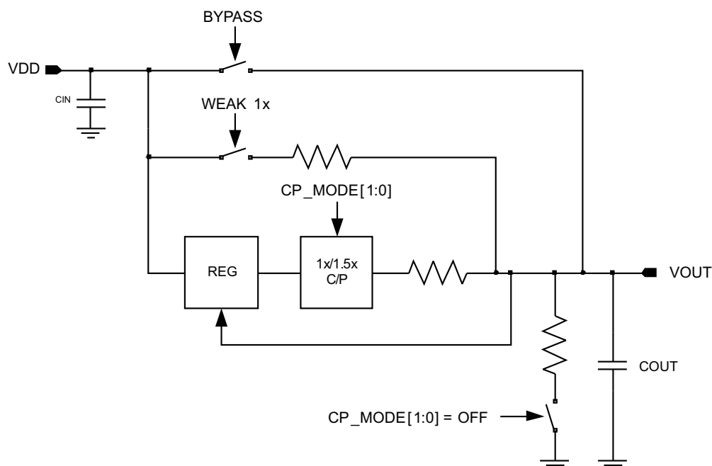
Figure 1. Functional Model of Charge Pump
