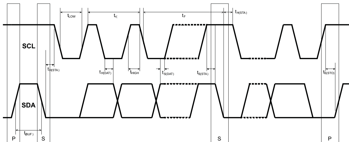
Figure 7. I²C Data Transmission Timing
