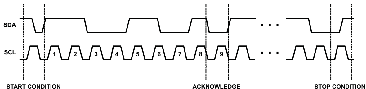
Figure 6. I²C Start / Stop / Acknowledge Protocol
