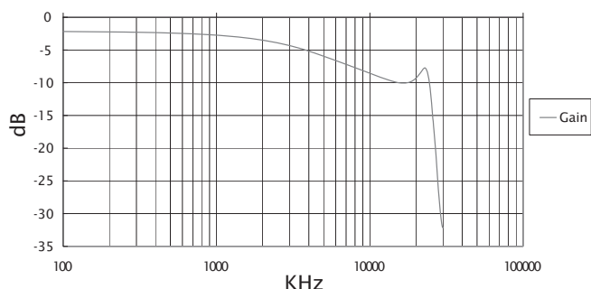
COMMON MODE
