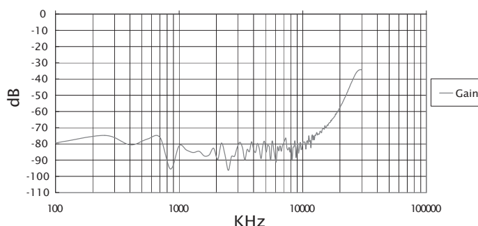
DIFFERENTIAL MODE
