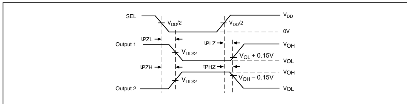
Voltage Waveforms Enable and Disable Times
