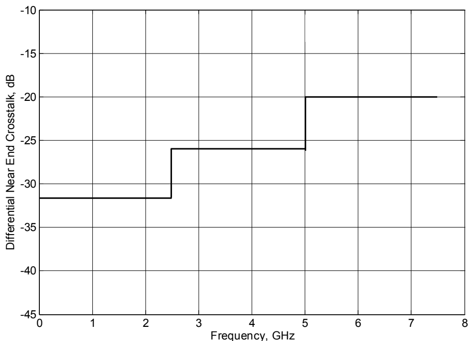
Figure 3: Illustration of differential near end crosstalk requirement.
