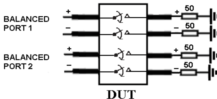
Differential Near End Crosstalk Test Circuit
