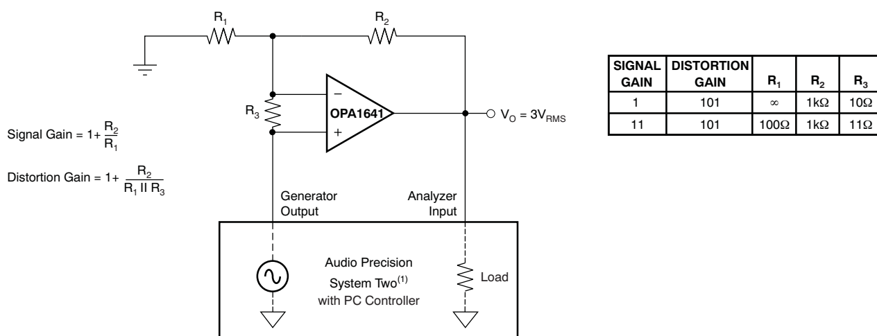
Figure 35. Distortion Test Circuit
