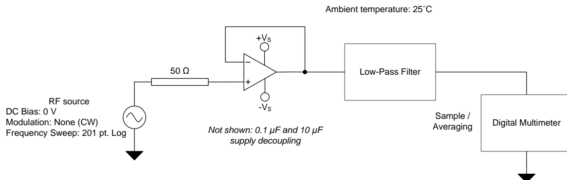
Figure 31. EMIRR IN+ Test Configuration Schematic
