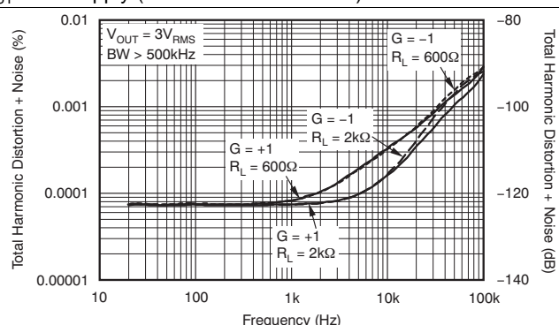
Figure 8. THD+N Ratio vs Frequency
