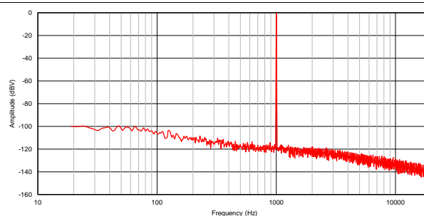
Figure 42. Output Spectrum for a 10 mV RMS , 1 kHz Input Signal
