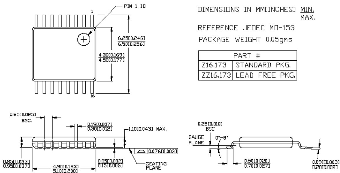
Figure 4. 16-Pin TSSOP 4.40 mm Body
