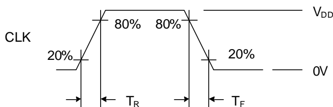
Figure 3. Output Rise and Fall Time
