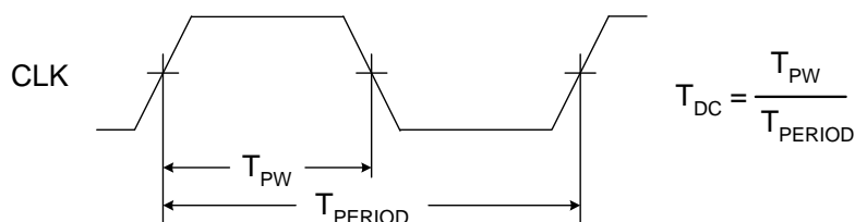
Figure 2. Output Duty Cycle Timing
