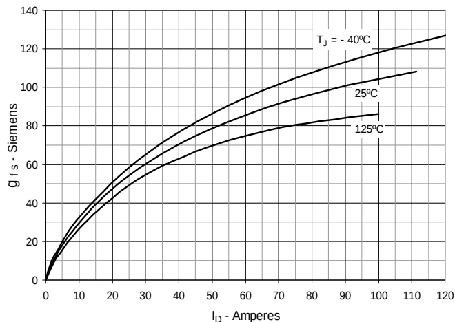
Fig. 8. Transconductance
