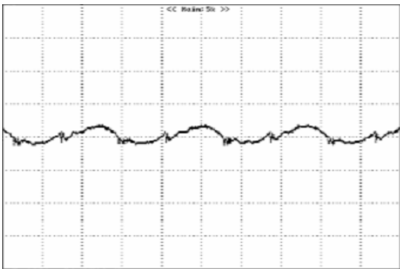
Figure 14: Output voltage ripple at nominal input voltage and rated load current ( I_o=20\text{A} ) ( 50\ \text{mV/div} , 1\ \mu\text{s/div} )
