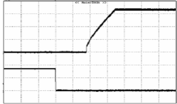
Figure 5: Turn-on transient at zero load current (5 ms/div). Vin=48V. Top Trace: Vout: 1.0V/div, Bottom Trace: ON/OFF input, 2V/div
