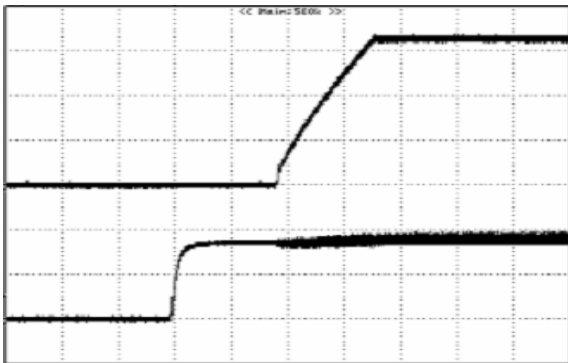
Figure 6: Turn-on transient at full rated load current (resistive load) (5 ms/div). Vin=48V. Top Trace: Vout, 1.0V/div; Bottom Trace: ON/OFF input, 2V/div
