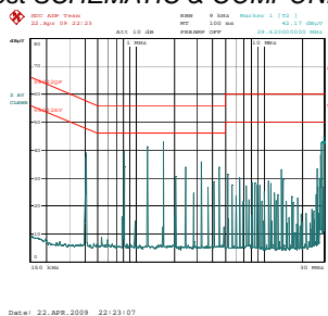
Fig17: EMI test result Vin = 48V Iout=20A AVERAGE
