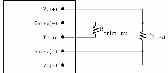
Figure 22: Circuit configuration for trim-up (increase output voltage)
