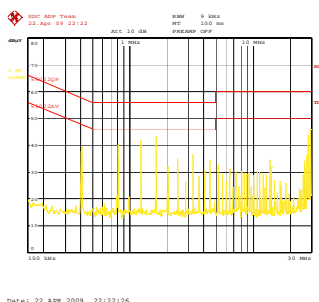
Fig18: EMI test result Vin = 48V Iout=20A Q.PEAK
