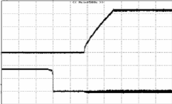
Figure 4: Turn-on transient at full rated load current (resistive load) (5 ms/div). Vin=48V. Top Trace: Vout, 1.0V/div; Bottom Trace: ON/OFF input, 2V/div
