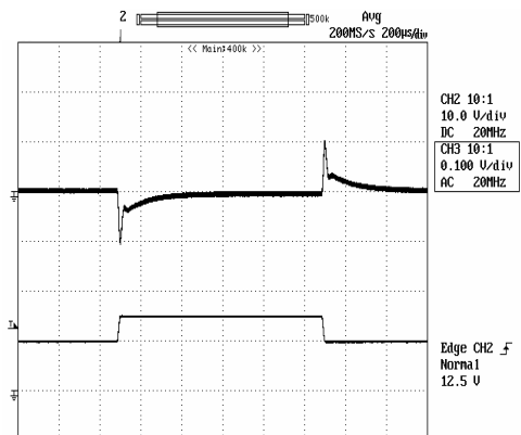
Figure 9: Output voltage response to step-change in load current (75%-50%-75% of I_o , max; di/dt = 1.0A/\mu s ). Load cap: 100 \mu F tantalum capacitor and 1 \mu F ceramic capacitor. Top Trace: Vout (100mV/div, 200us/div), Bottom Trace: Iout (10A/div). Scope measurement should be made using a BNC cable (length shorter than 20 inches). Position the load between 51 mm to 76 mm (2 inches to 3 inches) from the module
