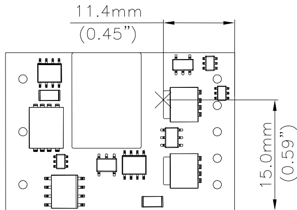
Figure 24: Temperature measurement location The allowed maximum hot spot temperature is defined at 123
