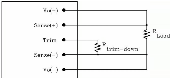
Figure 21: Circuit configuration for trim-down (decrease output voltage)
