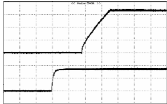
Figure 7: Turn-on transient at zero load current (5 ms/div). Vin=48V. Top Trace: Vout, 1.0V/div; Bottom Trace: ON/OFF input, 2V/div
