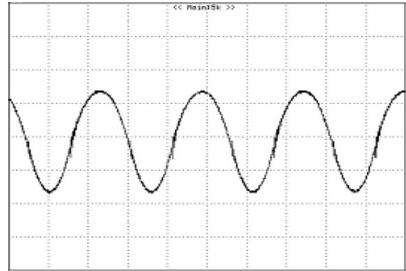
Figure 11: Input Terminal Ripple Current, i_c , at full rated output current and nominal input voltage with 12\ \mu\text{H} source impedance and 33\ \mu\text{F} electrolytic capacitor ( 200\ \text{mA/div} , 1\ \mu\text{s/div} )
