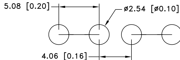
MOUNTING DETAIL
