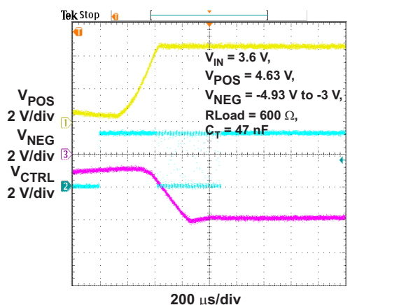
Figure 5. NEGATIVE OUTPUT VOLTAGE PROGRAMMING (Device enabled (CTRL = 400μs high), programmed to -3.0V)
