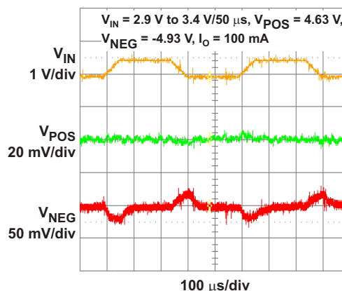
Figure 10. LINE TRANSIENT RESPONSE (100mA)
