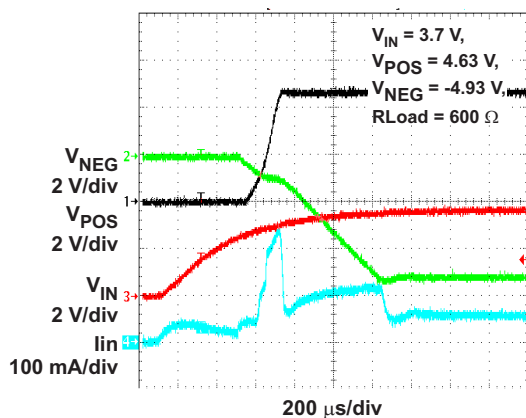
Figure 11. STARTUP
