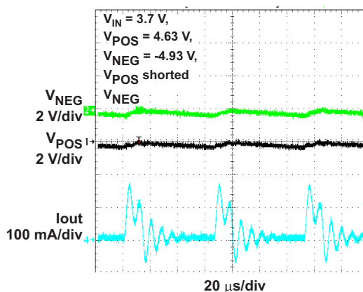
Figure 13. SHORT CIRCUIT
