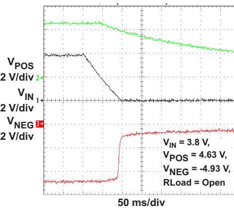
Figure 12. SHUTDOWN
