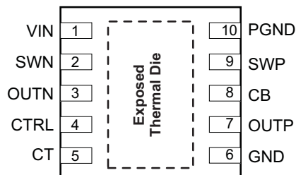
10 PIN TQFN PACKAGE (TOP VIEW)
