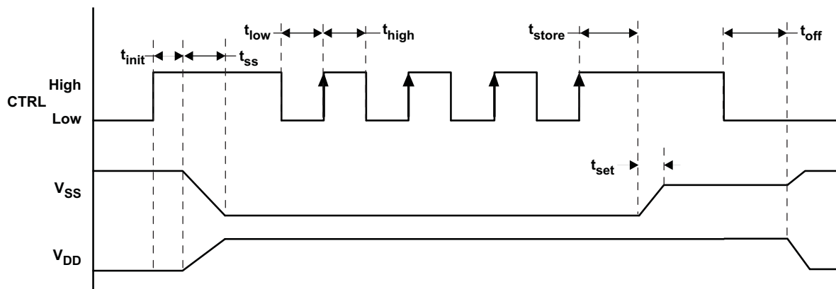
Figure 16. Digital Interface Using CTRL
