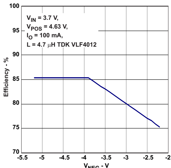
Figure 3. EFFICIENCY
