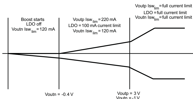
Figure 14. Soft Start and Short Circuit Thresholds
