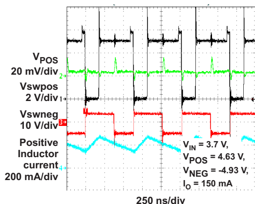
Figure 7. NOMINAL LOAD CURRENT OPERATION (VIN = 3.7V)
