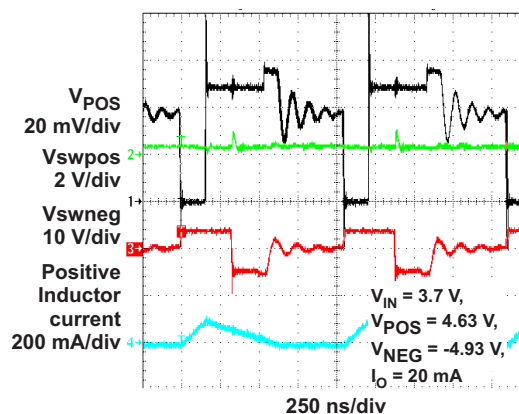
Figure 6. LIGHT LOAD CURRENT OPERATION
