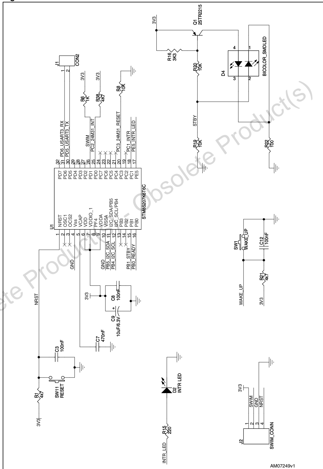
Figure 1. STEVAL-ILL029V: microcontroller
