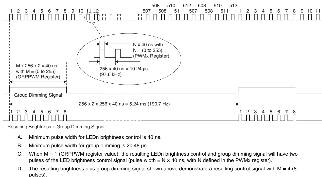
Figure 7. Brightness and Group Dimming Signals
