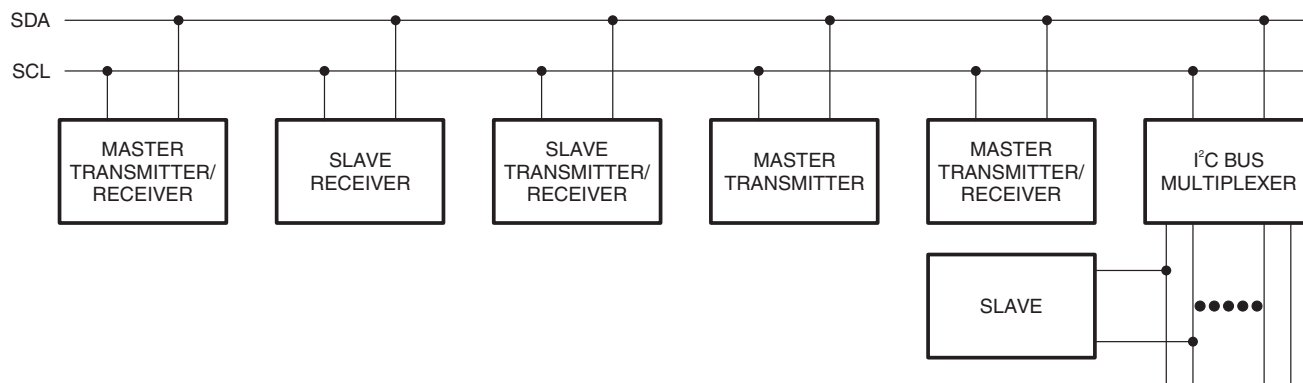
Figure 12. System Configuration
