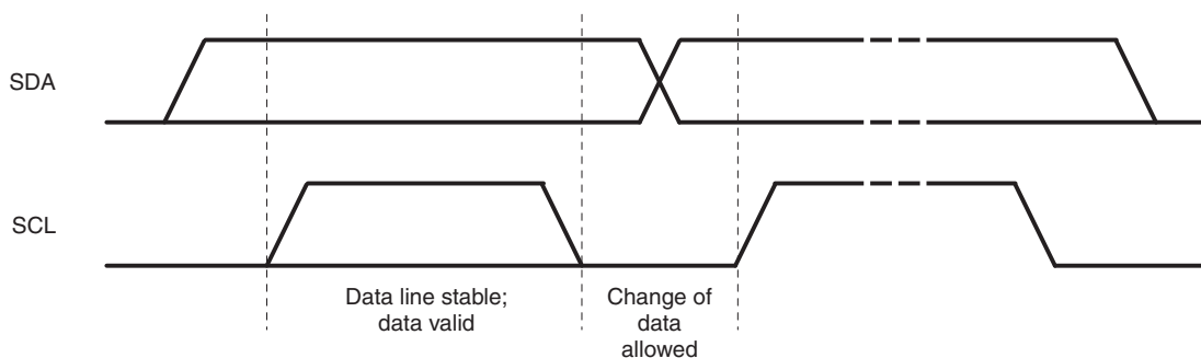
Figure 10. Bit Transfer
