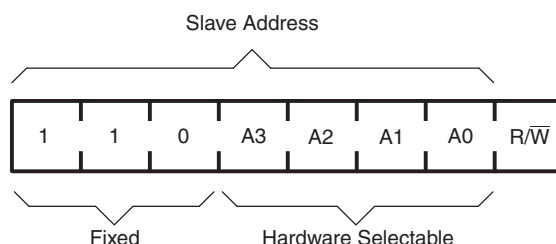
Figure 8. Slave Address
