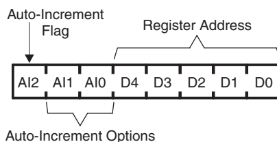
Figure 19. Control Register
