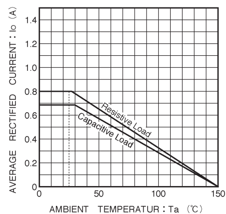
Fig. 3 Derating curve
