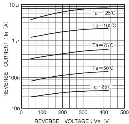
Fig. 2 Reverse characteristics
