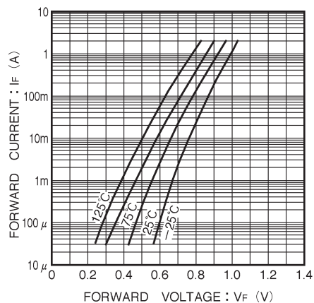
Fig. 1 Forward characteristics
