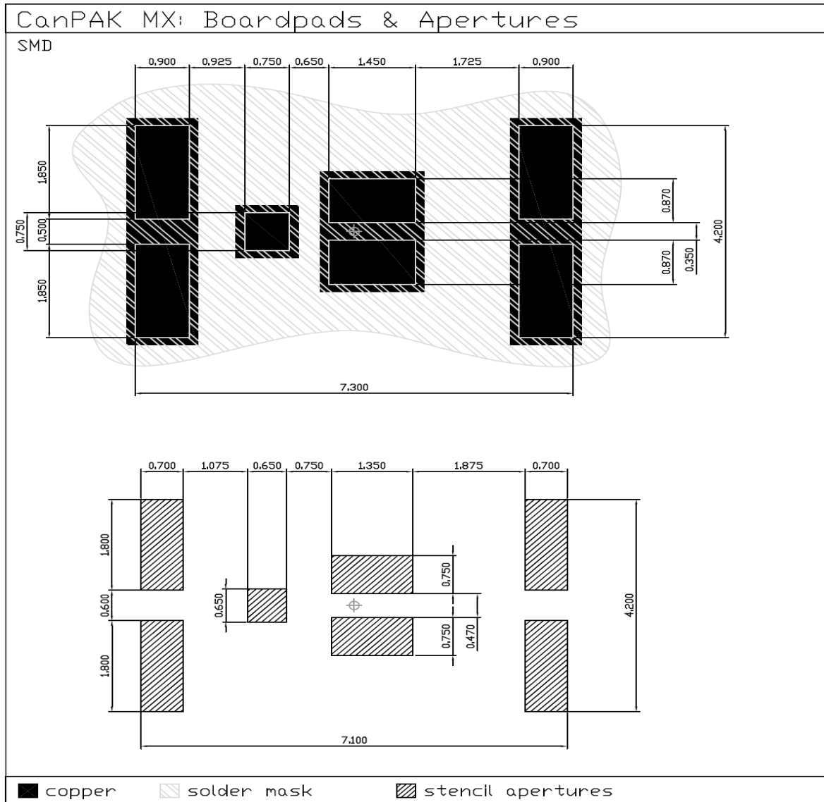
Figure 3 Outlines MG-WDSO-2, dimensions in mm/ Recommended stencil thickness 150µm
