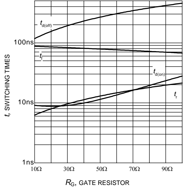
Figure 10. Typical switching times as a function of gate resistor (inductive load, T_J=175^\circ\text{C} , V_{CE} = 400\text{V} , V_{GE} = 0/15\text{V} , I_C = 6\text{A} , Dynamic test circuit in Figure E)
