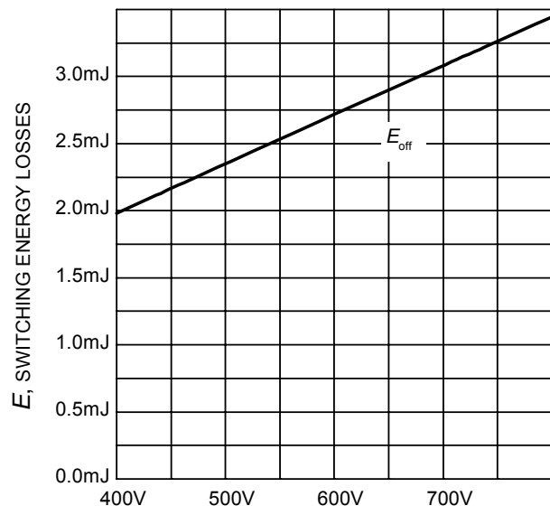
Figure 16. Typical switching energy losses as a function of collector emitter voltage (inductive load, T_J = 175^\circ\text{C} , V_{GE} = 0/15\text{V} , I_C = 30\text{A} , R_G = 26.9\Omega , Dynamic test circuit in Figure E)
