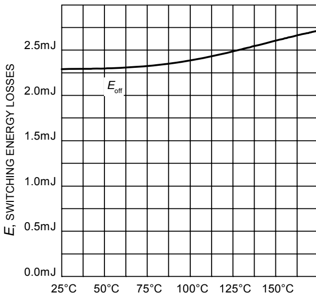
Figure 15. Typical switching energy losses as a function of junction temperature (inductive load, V_{CE} = 600\text{V} , V_{GE} = 0/15\text{V} , I_C = 30\text{A} , R_G = 26.9\Omega , Dynamic test circuit in Figure E)
