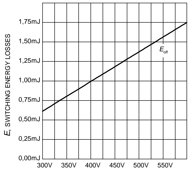
Figure 16. Typical switching energy losses as a function of collector emitter voltage (inductive load, T_J = 175^\circ\text{C} , V_{GE} = 0/15\text{V} , I_C = 30\text{A} , r_G = 10\Omega , Dynamic test circuit in Figure E)
