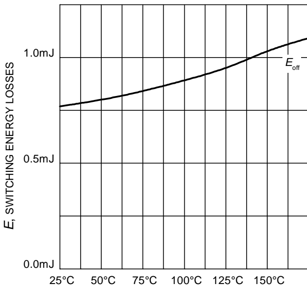
Figure 15. Typical switching energy losses as a function of junction temperature (inductive load, V_{CE} = 400\text{V} , V_{GE} = 0/15\text{V} , I_C = 30\text{A} , r_G = 10\Omega , Dynamic test circuit in Figure E)
